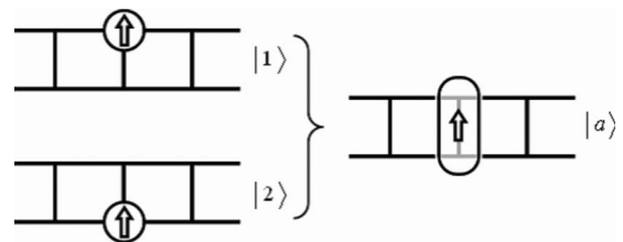
FIG. 1. Two states |1\rangle and |2\rangle represent CO states where a 3d^1 electron with up spin is located on a site. A 3d^1 electron shared within a rung is denoted as |a\rangle in Eq. (1). The arrows in the figure represent spins with S=1/2 .
