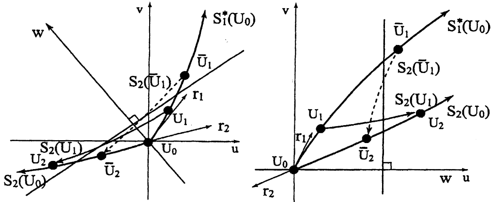
The situation for \text{sgn}(d\lambda_2 \cdot \hat{r}_2) = 1 .
