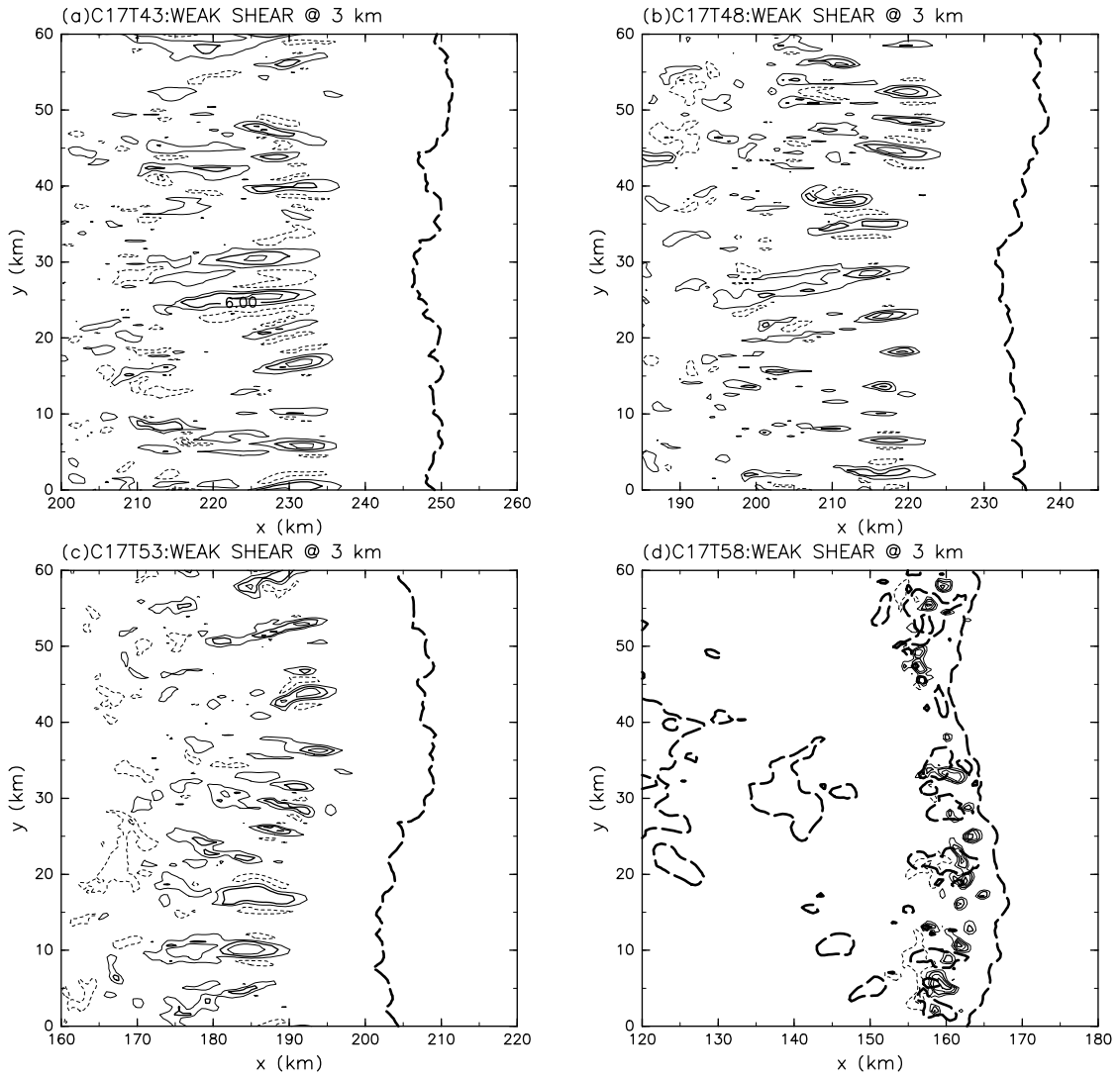
Figure 5: The same as Fig. 4, except for vertical velocity (contoured at 3-m s -1 interval).
