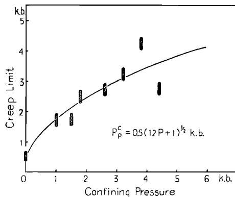
Fig. 7. Variation of the estimated creep limit with confining pressure for Kitashirakawa granite, at room temperature.
