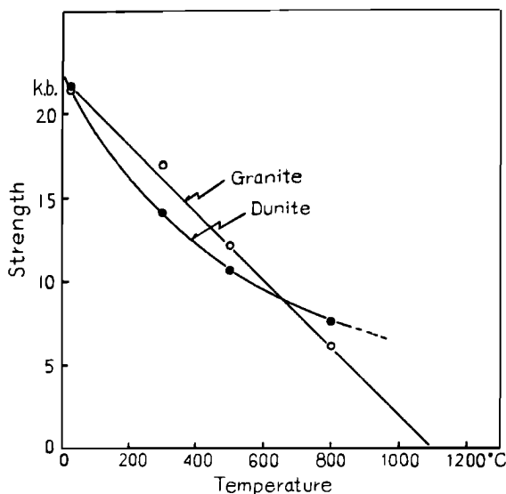
Fig. 3. Variation of strength of granite and dunite with temperature, at 5.0 k.b. confining pressure (after D. T. Griggs et al.).
