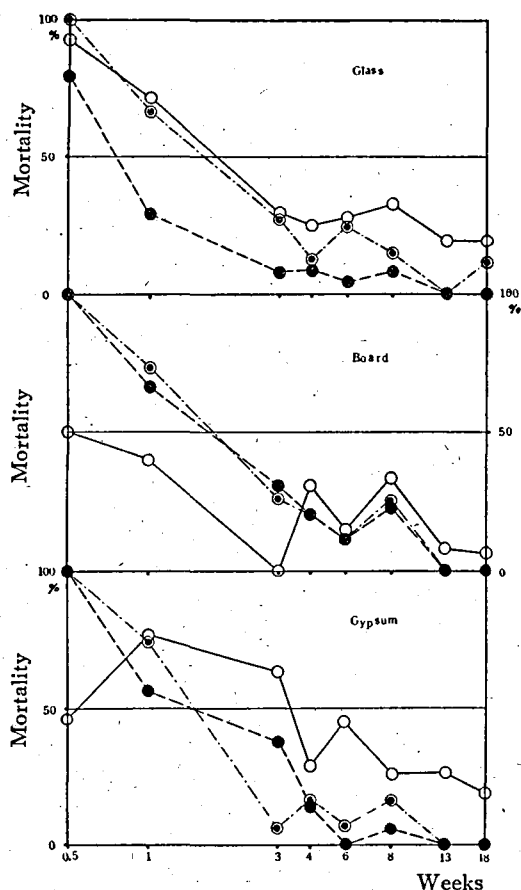
Fig. 3. The residual effect of insecticidal solutions applied on glass, board or gypsum to the common house fly. Mortality after 24 hours is shown. —○— indicates DDT, ----●---- lindane and - - -○- - - lindane B. The dosage is 200mg/ft 2 in DDT, or 20mg/ft 2 in lindane. (Exp. III)
