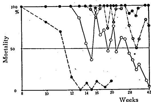
Fig. 1. The residual effect of insecticidal solution on glass to the common house fly. Mortality after 24 hours is shown. —○— indicates DDT, ---●--- lindane, ---○--- lindane A and ....●.... lindane B. The dosage is 500mg/ft 2 in DDT, or 50mg/ft 2 in lindane. (Exp. I)
