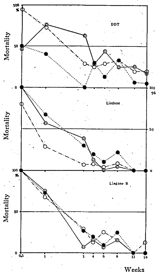
Fig. 4. Comparison of the persistence of the insecticidal residue. The data are based on the mortality after 24 hours listed in Table 3 (Exp. III). ----○---- indicates glass, ....●.... board and —○— gypsum.
