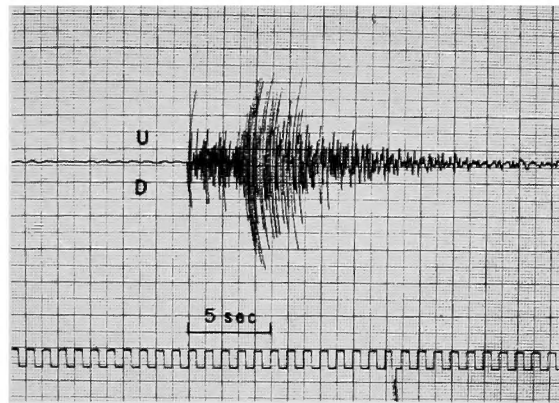
Fig. 8. An example of reproduced record of an earthquake whose initial motion was downward.
