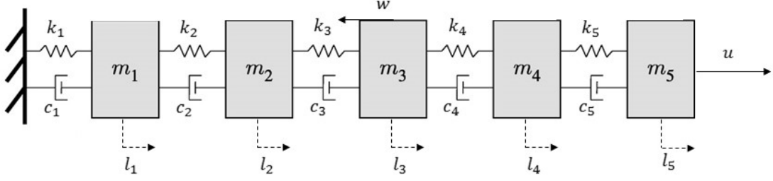
Figure 2. 5-mass-spring-damper system.
