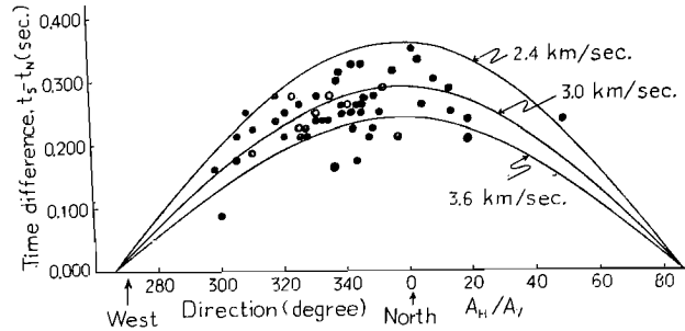
Fig. 19. Differences of the arrival times of microseismic waves at the two points of observation versus the arrival directions.
