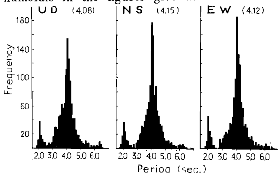
Fig. 3. Frequency distributions of the period of microseismic waves. The numerals show mean values of periods in each component.
