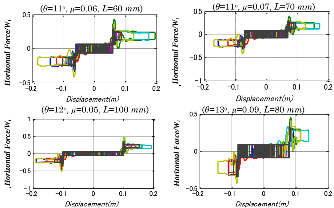
Figure 7.22 Time history analysis for design cases with moderate inclination angles
