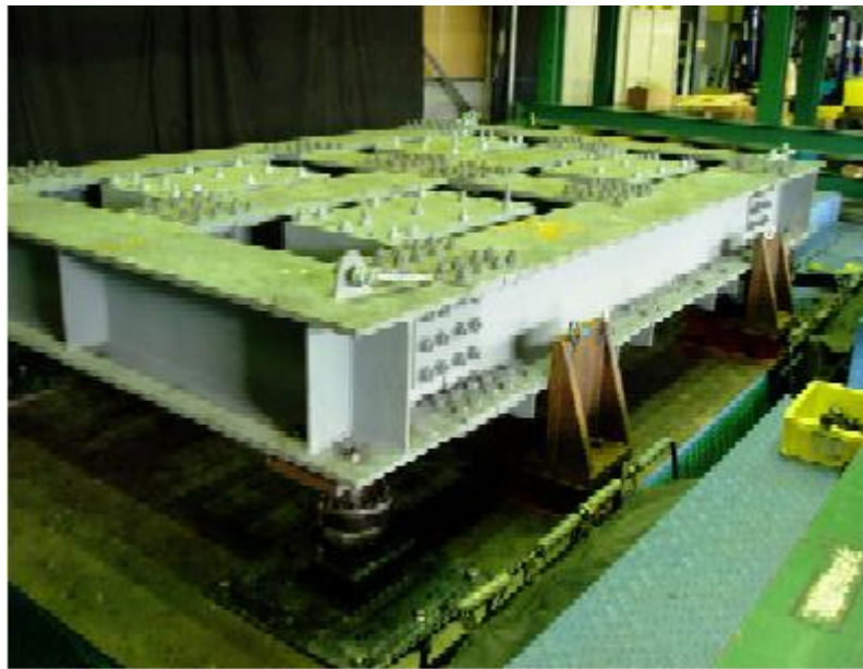
Figure 5.8 Experimental setup
