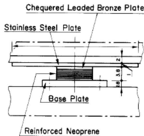
Figure 2.6 EDF isolator system
