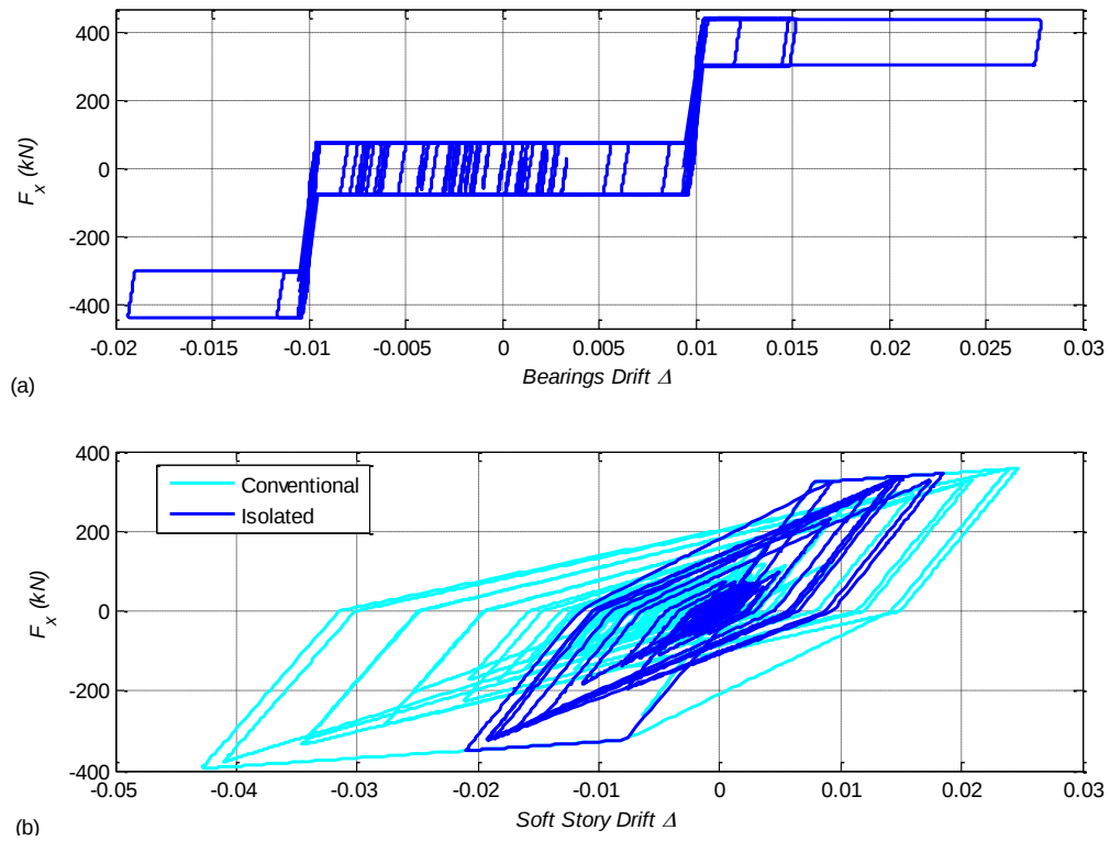
Figure 6.12 Hysteresis loop – El Centro record (a) the UPSS bearings (b) soft first story
