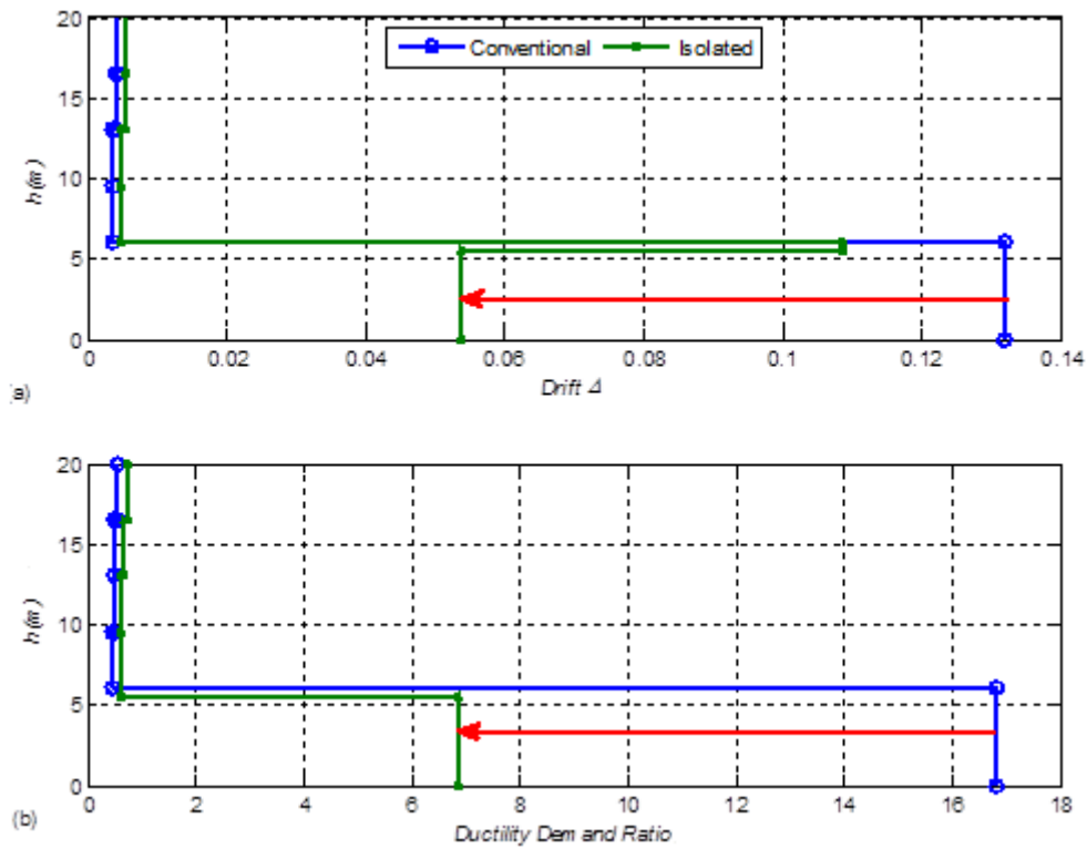
Figure 6.11 Comparison between conventional design and proposed isolation system subjected to Kobe record (a) max. story drift vs. story height (b) story ductility demand vs. story height
