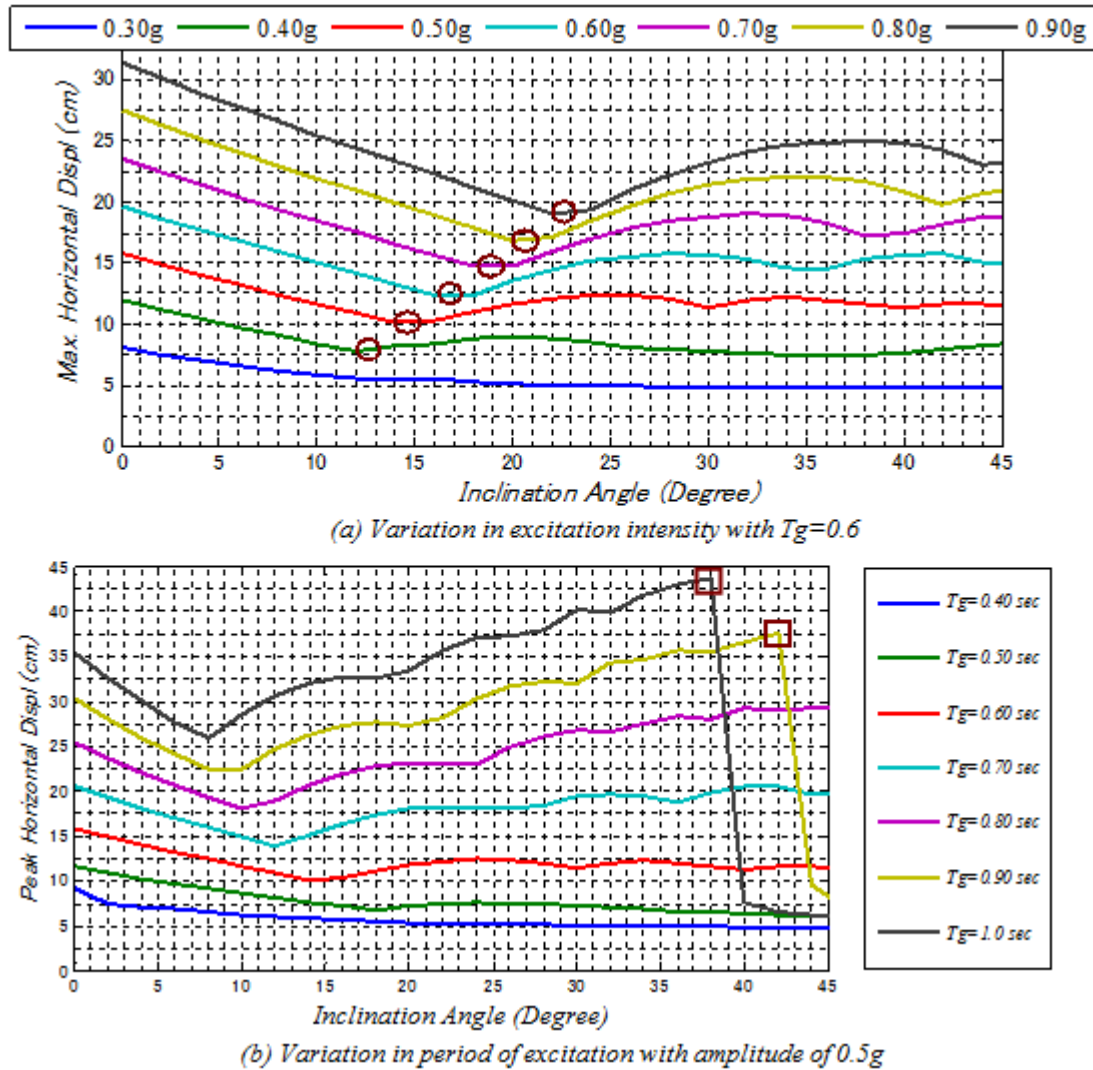
Figure 4.8 Maximum base horizontal displacement versus inclination angle
