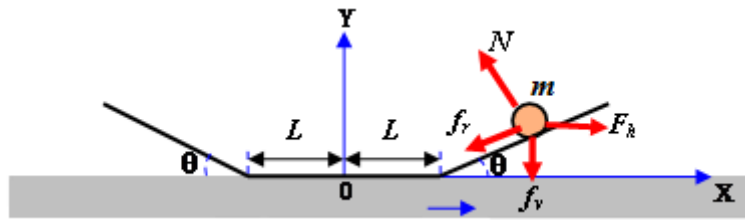
Figure 2.19 Mechanical model of the UPSS bearing
