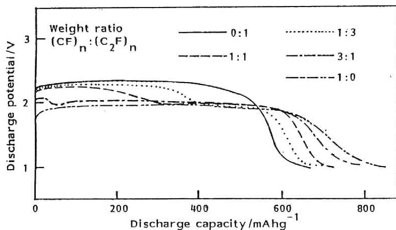
(A) Mixed electrodes of (CF)_n and (C_2F)_n
