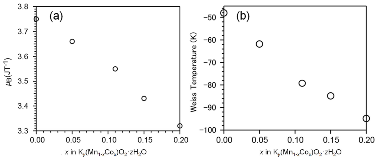
Figure 2.11. Variation of magnetic moment, \mu_B , with a composition x ( 0 \leq x \leq 0.2 ).
