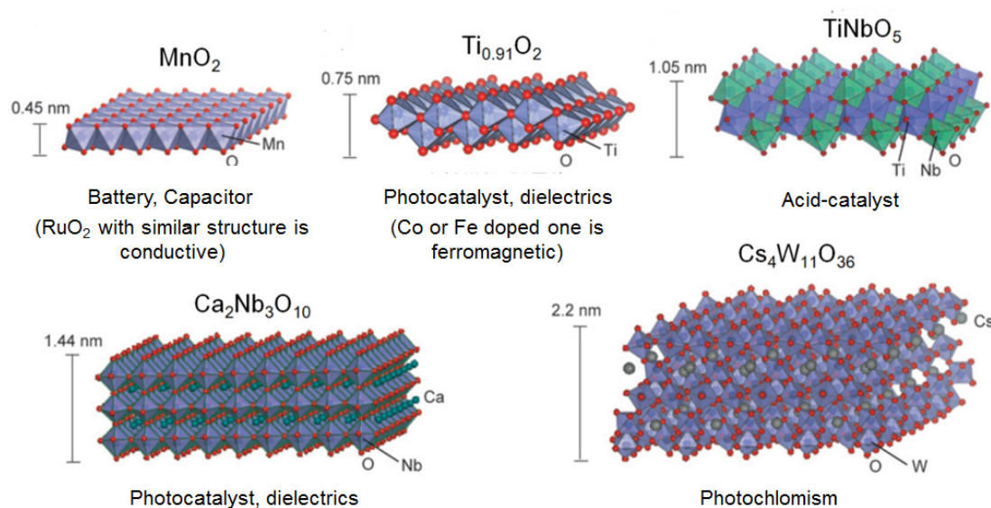
Figure 4. Representative structures of various functional nanosheets
