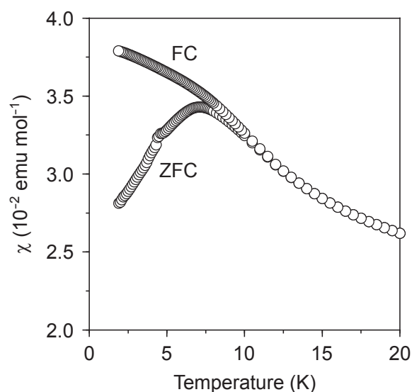
Figure 1.15. Temperature dependence of DC magnetic susceptibility ( \chi ) of \text{K}_{0.45}\text{MnO}_2 \cdot \text{H}_2\text{O} obtained by the sintering method. An applied magnetic field is 1 kOe. Spin glass behavior was observed as colloidal aggregate TMA/ \text{MnO}_2 (Fig. 1.14).
