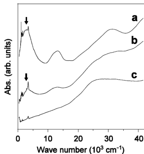
Figure 1.8. UV-Vis spectra of (a) starting material (\text{BEDO-TTF})_2\text{BF}_4 , (b) self-assembled organic-inorganic layered hybrid \text{BEDO-TTF}/\text{MnO}_2 , and (c) dried aggregate \text{TMA}/\text{MnO}_2 measured in compressed KBr pellets. A broad absorption band at around 4,000\text{ cm}^{-1} (arrows) is ascribed to the intermolecular transition between partially-charged BEDO-TTF molecules.
