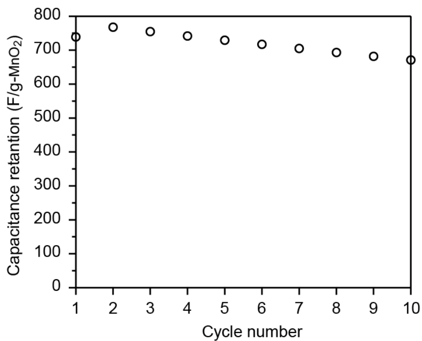
Figure 5.6. Cyclability of \text{MnO}_2/\text{AB} composite at a scan rate of 1 mV/s.
