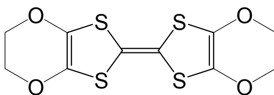
BEDO-TTF
