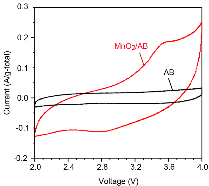
Figure 5.5. Cyclic voltammograms of AB and \text{MnO}_2/\text{AB} composite at a scan rate of 1 mV/s
