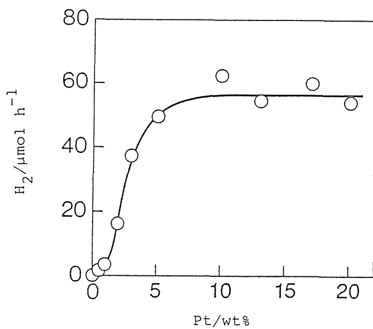
Figure 8 Dependence of the photocatalytic activity of \text{TiO}_2 ( T_c = 700^\circ\text{C} ) on Pt loading.
