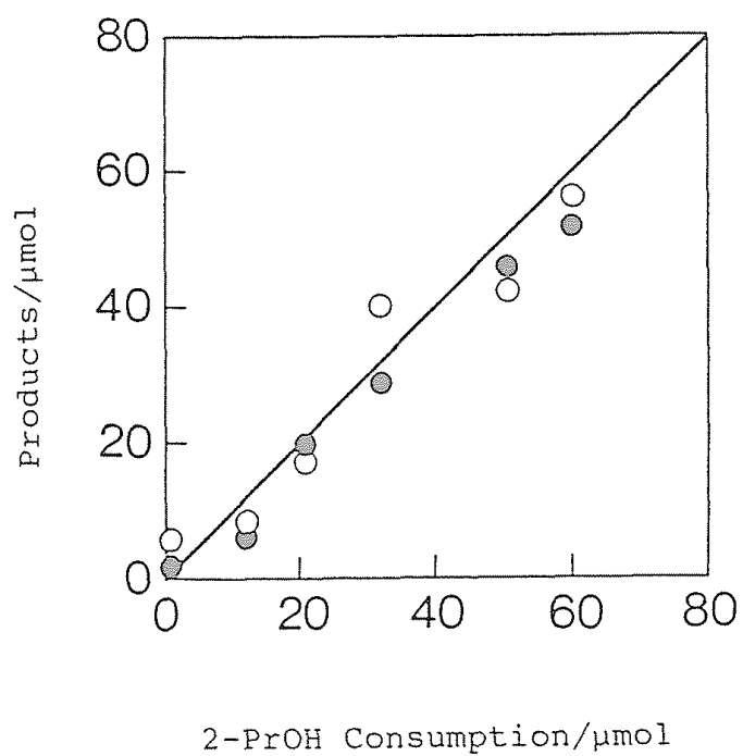
Figure 7 Material balance in the \text{TiO}_2/\text{Pt} (5 wt%)/2-PrOH aq. photoreaction system (1 h irradiation); ○ : \text{H}_2 , ● : Acetone.
