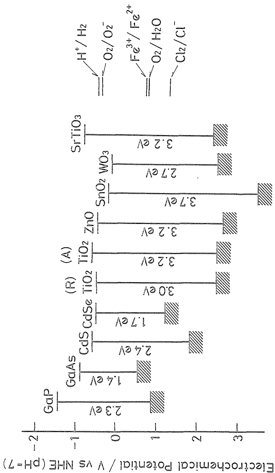
Scheme 2 Potential of conduction and valence bands of various semiconductors; (A) and (R) show anatase and rutile \text{TiO}_2 , respectively.
