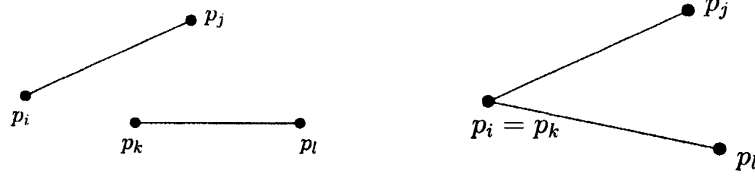
Figure 1: (p_i, p_j) < (p_k, p_l) .
