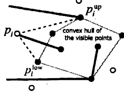
Figure 2: An example of the upper and lower tangents, denoted by (p_i, p_i^{up}) and (p_i, p_i^{low}) , respectively. The bold edges represent S .
