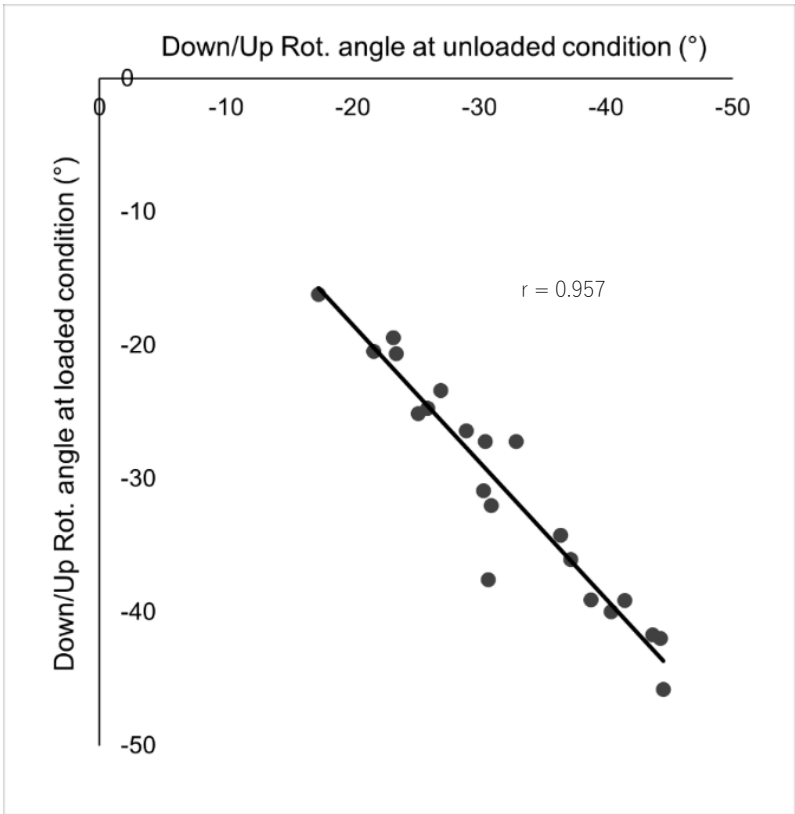
338 Figure S2. scatterplot of loaded vs. unloaded at the instant of maximum absolute r-value 339
