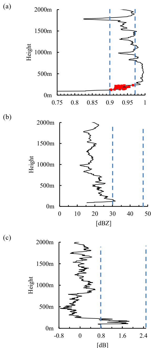
Fig. 8 Example of (a) \rho_{HV} , (b) Z_H and (c) Z_{DR} distribution in the radial direction at an azimuth. Freezing level is 405m observed by sonde. Red points of (a) are detected ML points. Blue dash lines are threshold values of each parameter.
