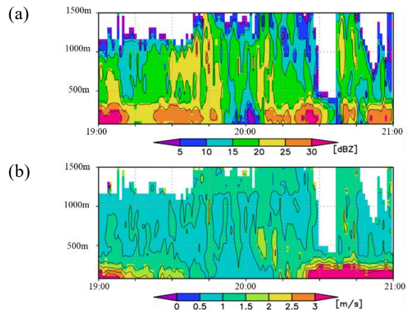
Fig. 15 2019/1/28 19:00-21:00. Vertical profile of (a) Z and (b) Fall velocity observed by micro rain radar installed ground observation point.
