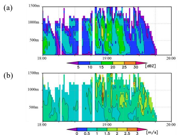
Fig. 16 2019/2/22 18:00-20:00. Vertical profile of (a) Z and (b) Fall velocity observed by micro rain radar installed ground observation point.
