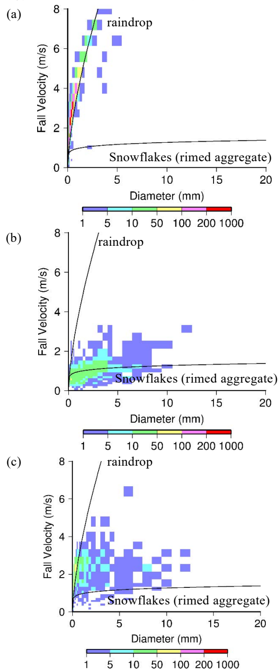
Fig. 13 Example of precipitation particle diameter – fall velocity distribution about (a) rainfall, (b) snowflakes and (c) wet snow. Curves correspond to empirical relationships for raindrop (Atlas et al., 1977) and snowflakes (Ishizaka, 1995).
