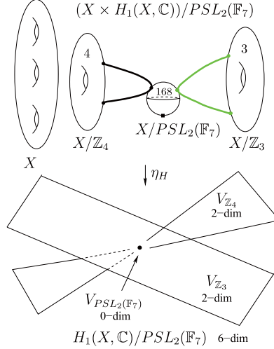
Figure 4.2: For the Klein curve X , its homological quotient family (X \times H_1(X, \mathbb{C}))/PSL_2(\mathbb{F}_7) \rightarrow H_1(X, \mathbb{C})/PSL_2(\mathbb{F}_7) has the above configurations of veins, fibers, and ridges.
