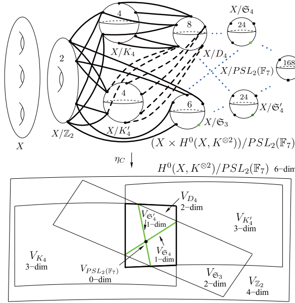
Figure 4.3: For the Klein curve X , its canonical quotient family (X \times H^0(X, K^{\otimes 2}))/PSL_2(\mathbb{F}_7) \rightarrow H^0(X, K^{\otimes 2})/PSL_2(\mathbb{F}_7) has the above configurations of veins, fibers, and ridges.
