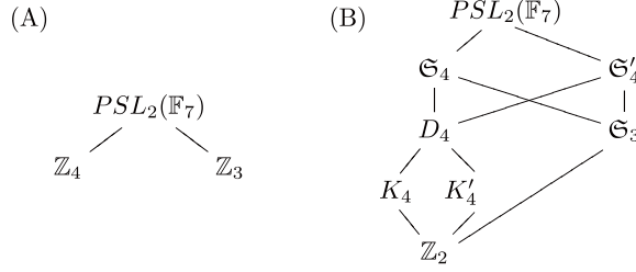
Diagram 4.4: (A) and (B) are the Hasse diagrams of stabilizers for the \text{Aut}(X) -actions on H_1(X, \mathbb{C}) and H^0(X, K^{\otimes 2}) . “ A - B ” means “ A \subset B ”.
