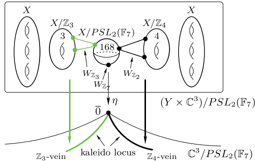
Figure 4.1: Linear quotient family of the Klein curve associated with \rho_3 .
