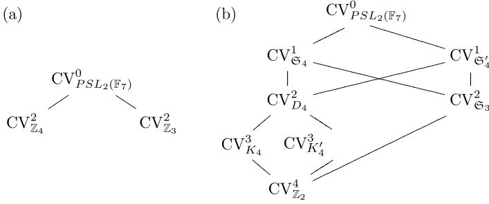
Diagram 4.5: (a) and (b) are the Hasse diagrams of conveyins for the \text{Aut}(X) -actions on H_1(X, \mathbb{C}) and H^0(X, K^{\otimes 2}) . CV^d_H means that the H -convein CV_H is of dimension d .
