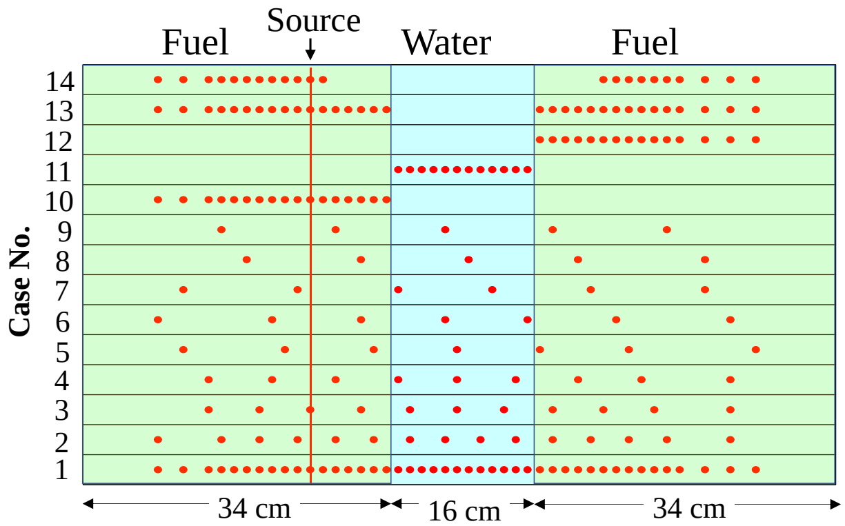
Fig. 13 Arrangements of detector positions for DMD (numerical data of detector positions are presented in an excel file as “Supplementary material”)
