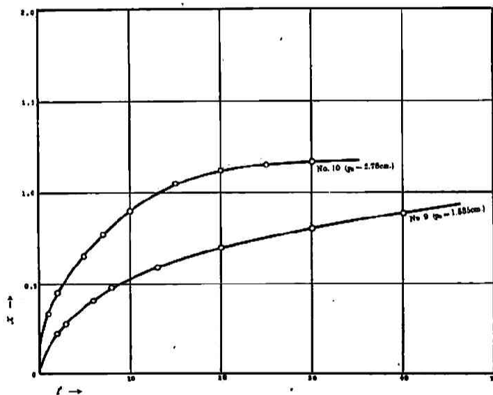
Fig. 5.—Expts. at 460°C. with activated Ni.
