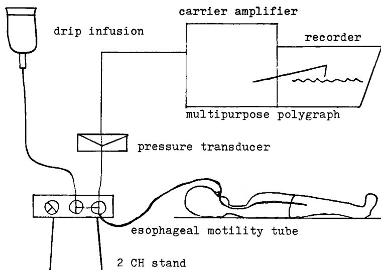
Fig. 1. Apparatus for esophageal manometry
