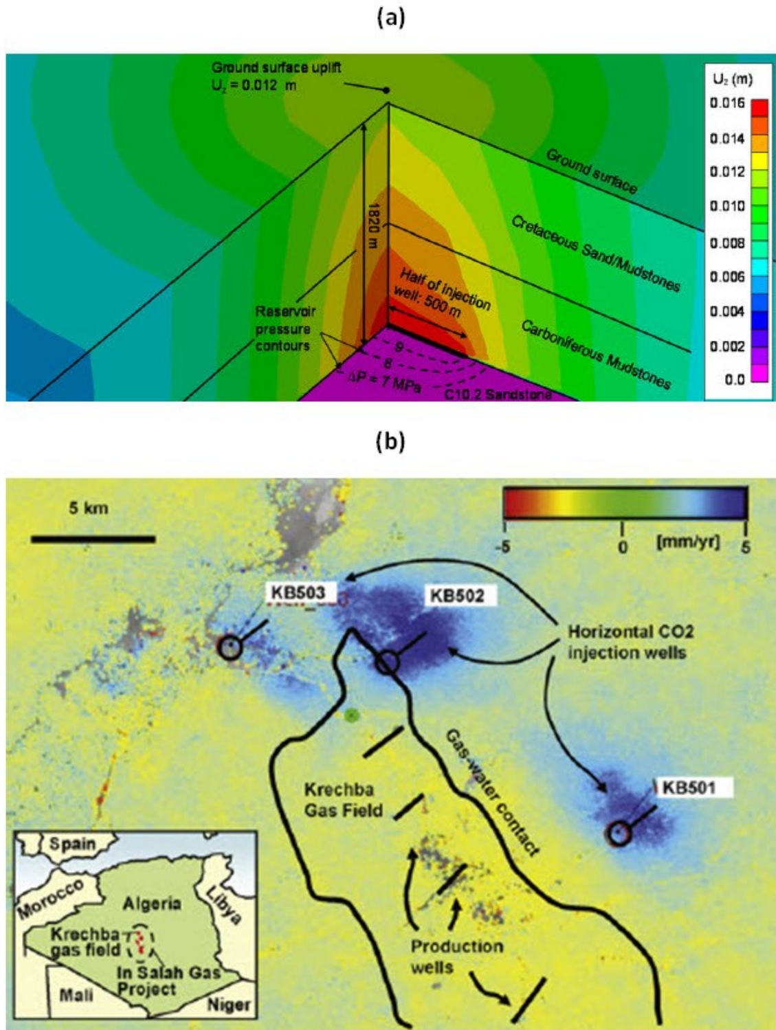
Figure 2.14 Surface uplift at In Salah, Algeria (a) The result from geomechanics simulation (b) The result from InSAR (Rutqvist, 2010)
