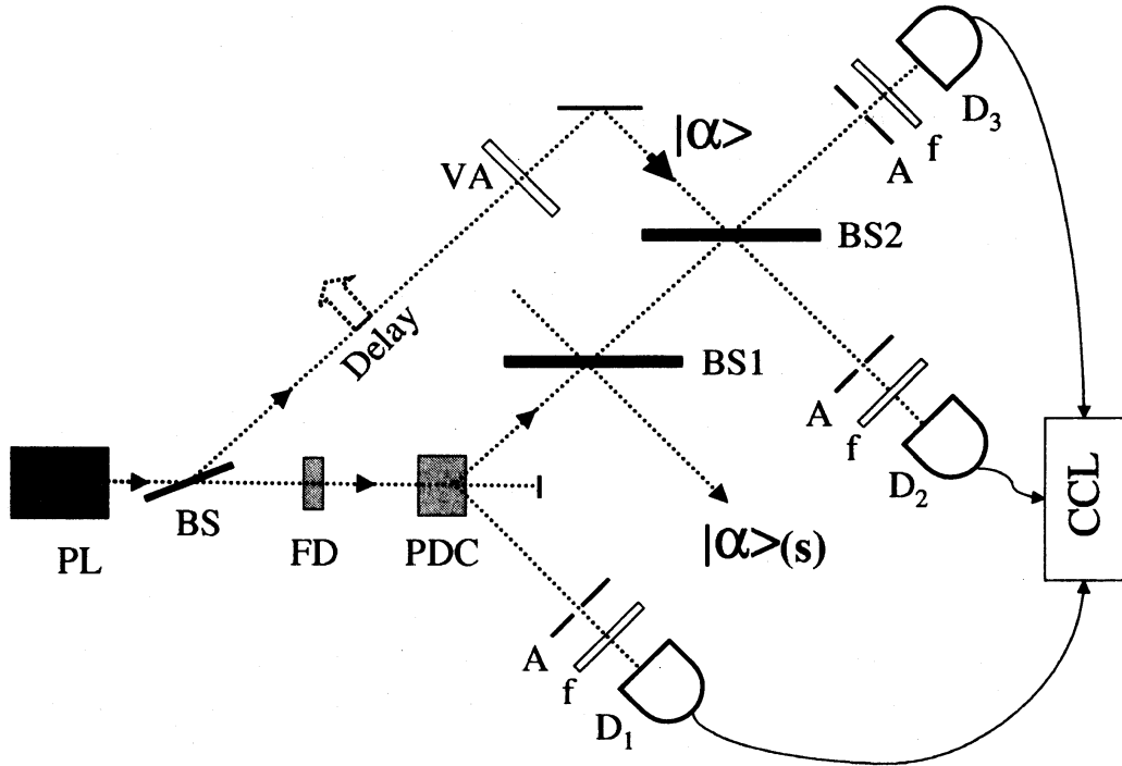
FIG. 2. Scheme of experimental realization of the PPB quantum scissors corresponding to Fig. 1(a). Key: PL – pulsed laser; FD – frequency doubler; PDC – parametric down conversion crystal; VA – variable attenuator; A – aperture; f – narrow band filter; CCL – coincidence counter and logic; BS, BS1, and BS2 – beam splitters; and D_1 , D_2 , and D_3 – photon-counting detectors.
