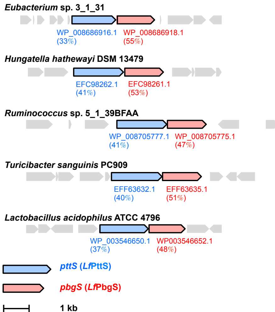
Fig. S8 Distribution of gene clusters containing pttS and pbgS homologues in gut bacteria. Genes encoding homologues of LfPttS and LfPbgS are colored blue and red, respectively. The GenBank accession number assigned to each gene encoding a LfPttS or LfPbgS homologue and its sequence identity obtained by TBLASTN analysis is shown below its coding region. All bacteria listed above are gut bacteria whose genomic sequences were obtained by metagenomic sequencing of gut microbiome in the Human Microbiome Project (31).
