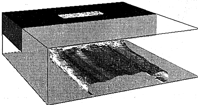
Figure 4: Profile of free surface (P_{in} = 1.35, V_{film} = 1.96)
