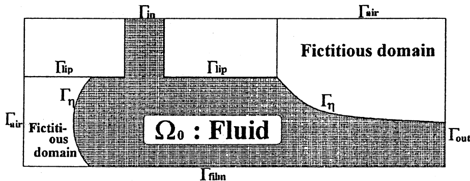
Figure 2: Projection of analyzed domain into x - z plane
