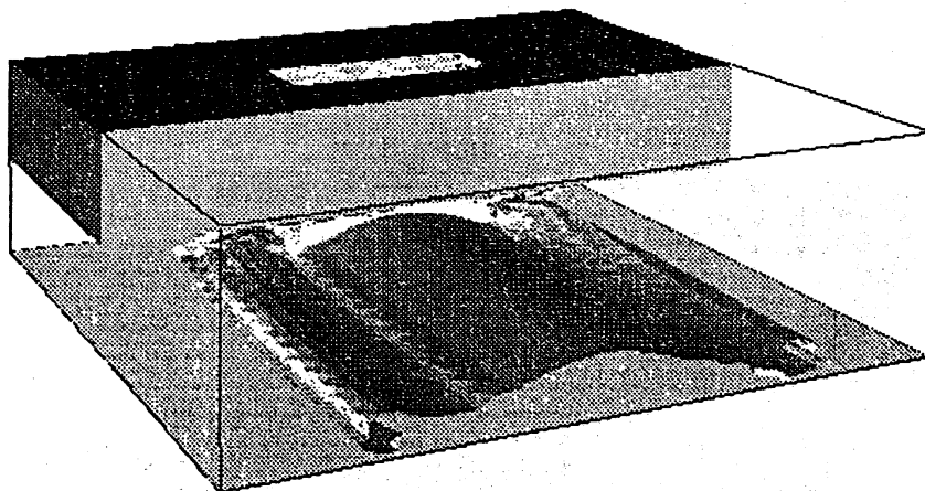
Figure 6: Profile of free surface ( P_{in} = 4.0, V_{film} = 4.0 )
