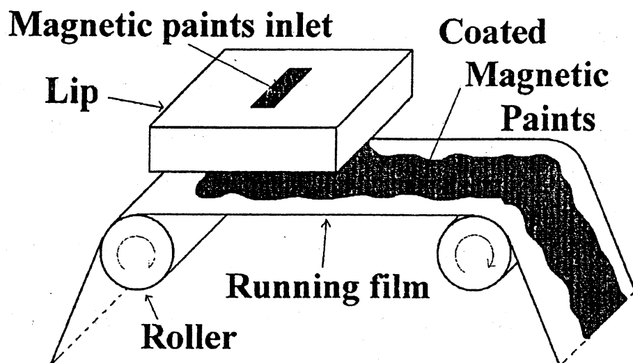
Figure 1: Coating process of magnetic paints
