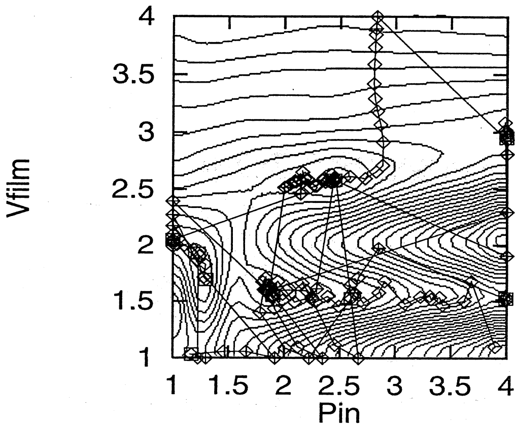
Figure 3: Contours of cost function and searching path by FOM-MCA
