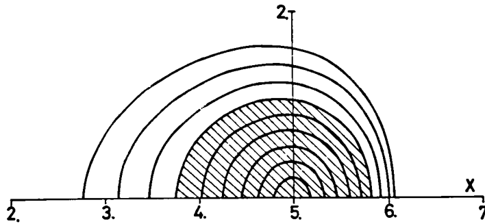
Fig.IV-6. Magnetic surfaces of Tokamak equilibrium with \beta_p = 3.0 , S_{2b} = 0.0 , S_{3b} = 0.4 and with the uniform toroidal current.
