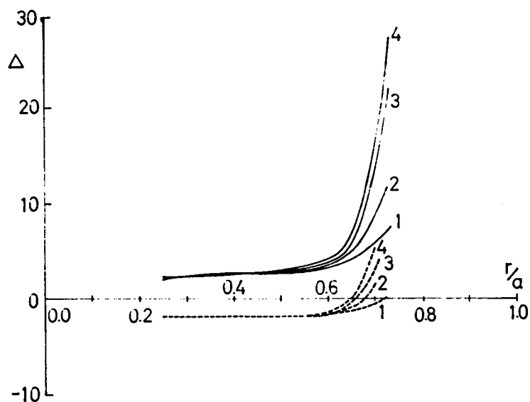
Fig.II-15. \Delta as a function of r/a when plasma pressure \beta changes for R_B = -0.15 , \alpha = 1.0 . Solid lines show m = 1 mode and dotted lines show m = 2 mode. 1) \beta = 15\% , 2) \beta = 20\% , 3) \beta = 26\% , 4) \beta = 31\% .
