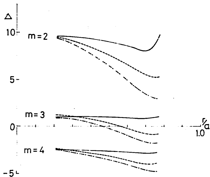
Fig.V-10. Variation of \Delta for the current profile J = J_0 \exp(-\kappa^2 r^2/a^2) in a plasma column surrounded by a vacuum; \beta = 1.5\% , q_a = 3.0 and the conducting shell is located at 1.5a . The solid line shows for \kappa = 1 , the dotted line for \kappa = \sqrt{2} and the dashed line for \kappa = \sqrt{3} .
