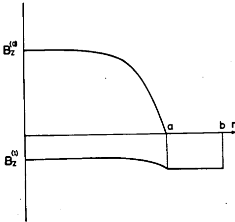
Fig.II-2. B_z^{(0)} and B_z^{(1)} which give a reverse field pinch.
