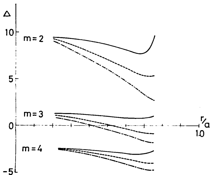
Fig.V-11. Variation of \Delta for the current profile J = J_0 \exp(-\kappa^2 r^2/a^2) in a plasma column surrounded by a vacuum; \beta = 1.5\% , q_a = 2.0 and the conducting shell is located at 1.5a . The solid line shows for \kappa = 1 , the dotted line shows for \kappa = \sqrt{2} and the dashed line for \kappa = \sqrt{3} .
