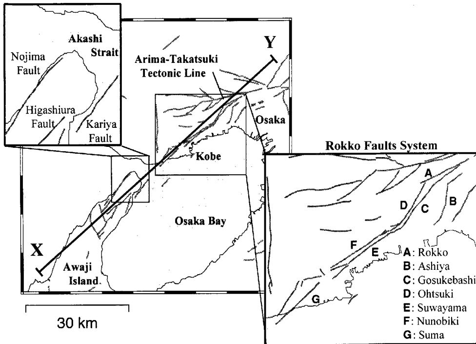
Fig. 1. The distribution of active faults. The Rokko Faults System is consist of active faults called (A) the Rokko Fault, (B) the Ashiya Fault, (C) the Gosukebashi Fault, (D) the Ohtsuki Fault, (E) the Suwayama Fault, (F) the Nunobiki Fault and (G) the Suma Fault respectively. Line X-Y shows the cross sections in Figures 8-11.
