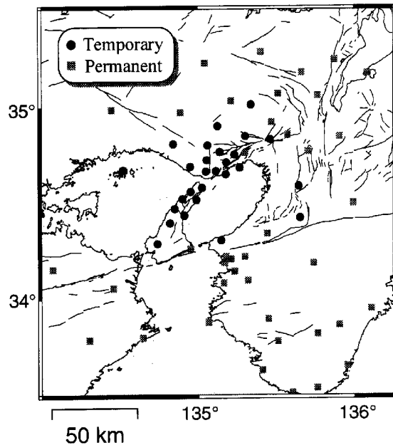
Fig. 2. Distribution of the seismic stations used in this study. Solid circles are temporary stations deployed by GROUPS-95 following the Hyogo-ken Nanbu earthquake. Gray squares are permanent stations.
