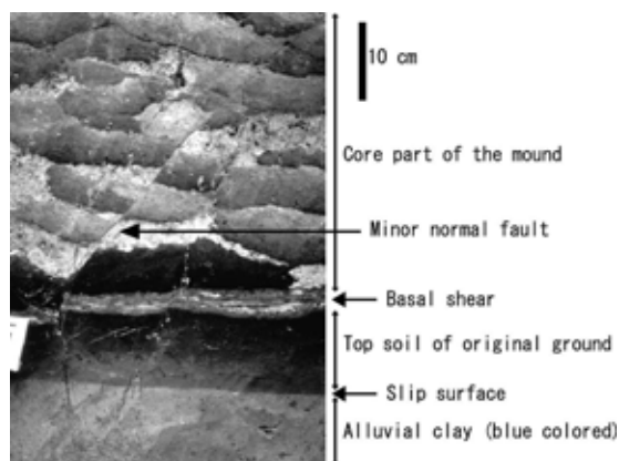
Fig.13 Shears of the landslide
