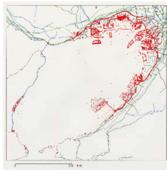
Fig. 2 Locations of boreholes in the Geotechnical Database in the Osaka Bay Area
