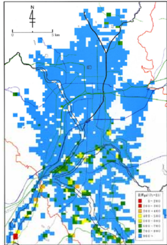
Fig. 4 Calculated Acceleration to Induce Liquefaction in terms of P_L=15 in Kyoto Basin
