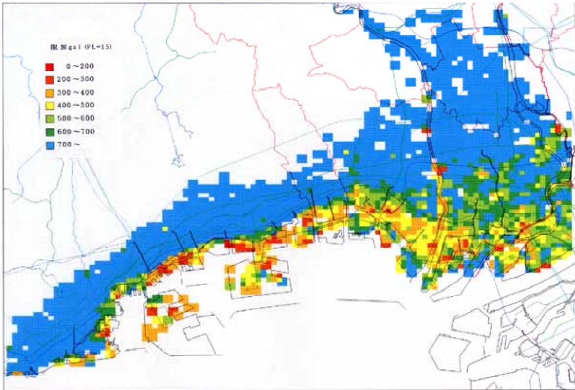
Fig. 5 Calculated Acceleration to Induce Liquefaction in terms of P_L=15 in Kobe to Hanshin Area
