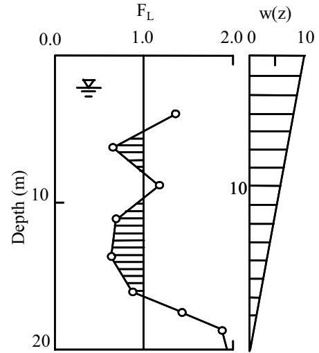
Fig. 3 Derivation of the Integrated Safety factor, P_L for Occurrence of Liquefaction
