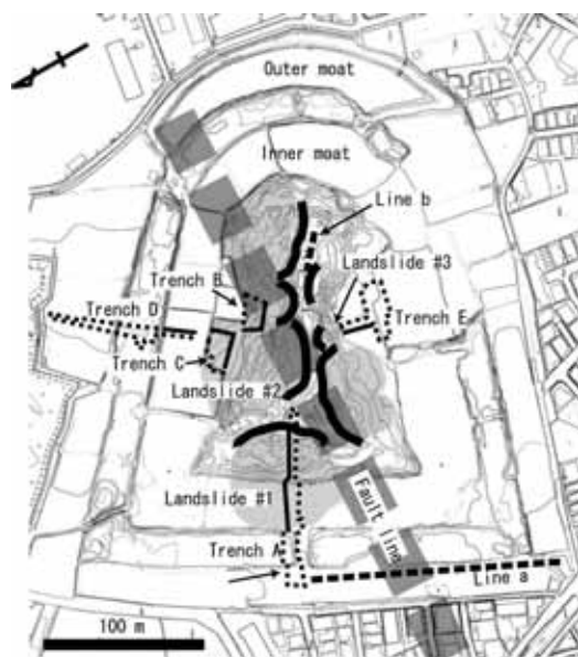
Fig.11 Landslides on the mound and earthquake fault in 1596
