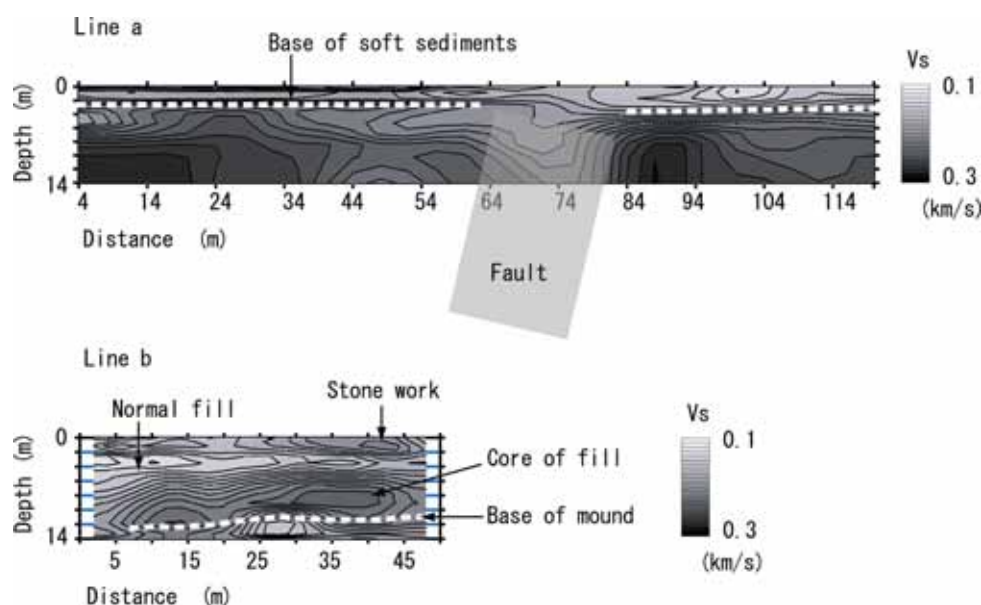
Fig.12 Vs cross-section of the mound
