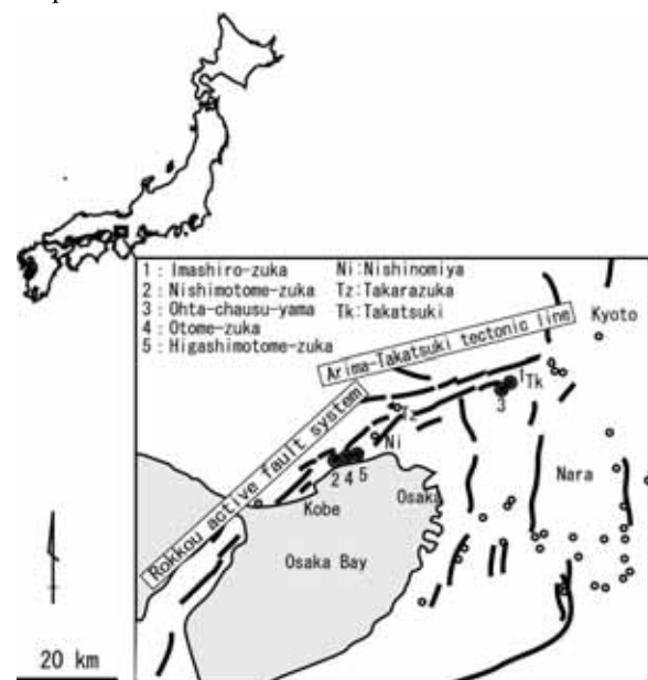
Fig.10 Distribution of ancient mounds and active fault system of the Kinki district
