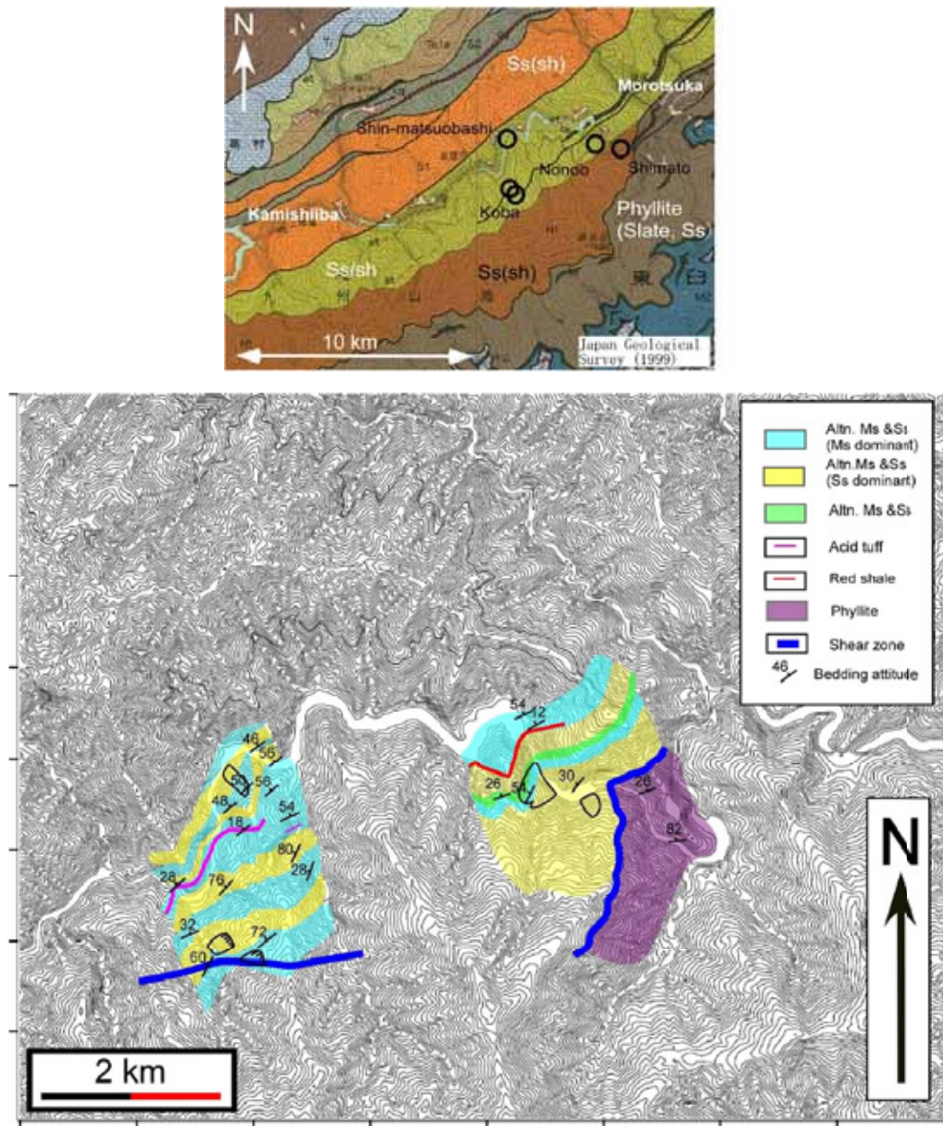
Fig. 6 Geologic map around large landslides along the Mimi River, central Kyushu. Circles with names indicate large landslide sites.
