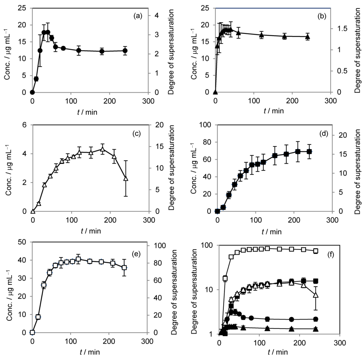
Figure 3.1. Concentration-time profiles of amorphous (a) danazol, (b) griseofulvin, (c) itraconazole, (d) vemurafenib and (e) ER-34122 in the dissolution test (left axis). The right axis shows the degree of supersaturation at each time point. The degree of supersaturation-time profiles for the five model drugs [danazol (●), griseofulvin (▲), itraconazole (Δ), vemurafenib (■) and ER-34122 (□)] are summarized in (f). Each value represents the mean \pm SD ( n = 3 ).
