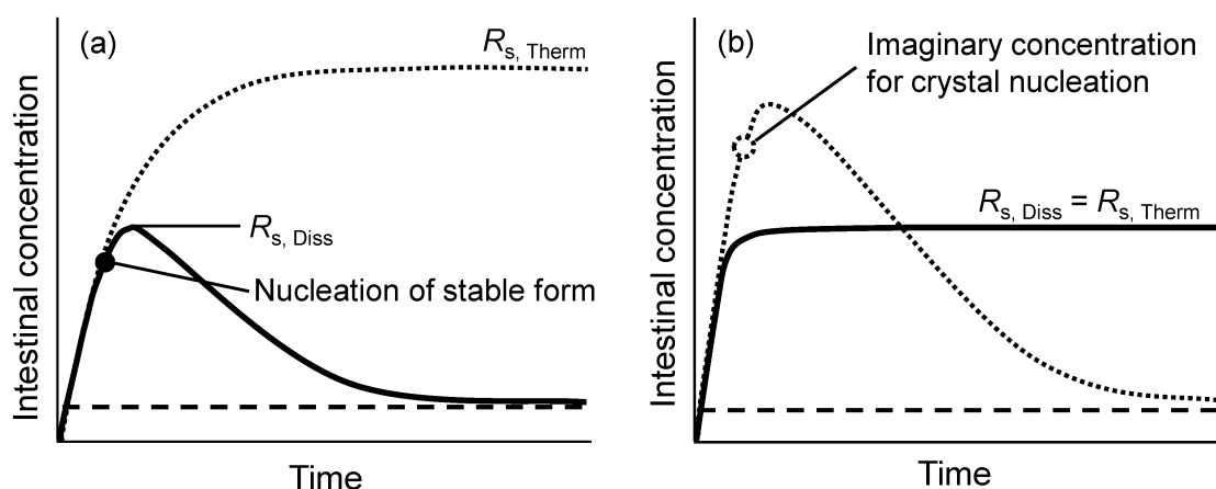
Figure 3.7. Schematic diagrams of (a) kinetically-controlled and (b) thermodynamically-controlled supersaturation of amorphous solids. Solid and dotted lines are actual and imaginary supersaturation profiles, respectively. Broken lines show the thermodynamic solubility of stable forms.
