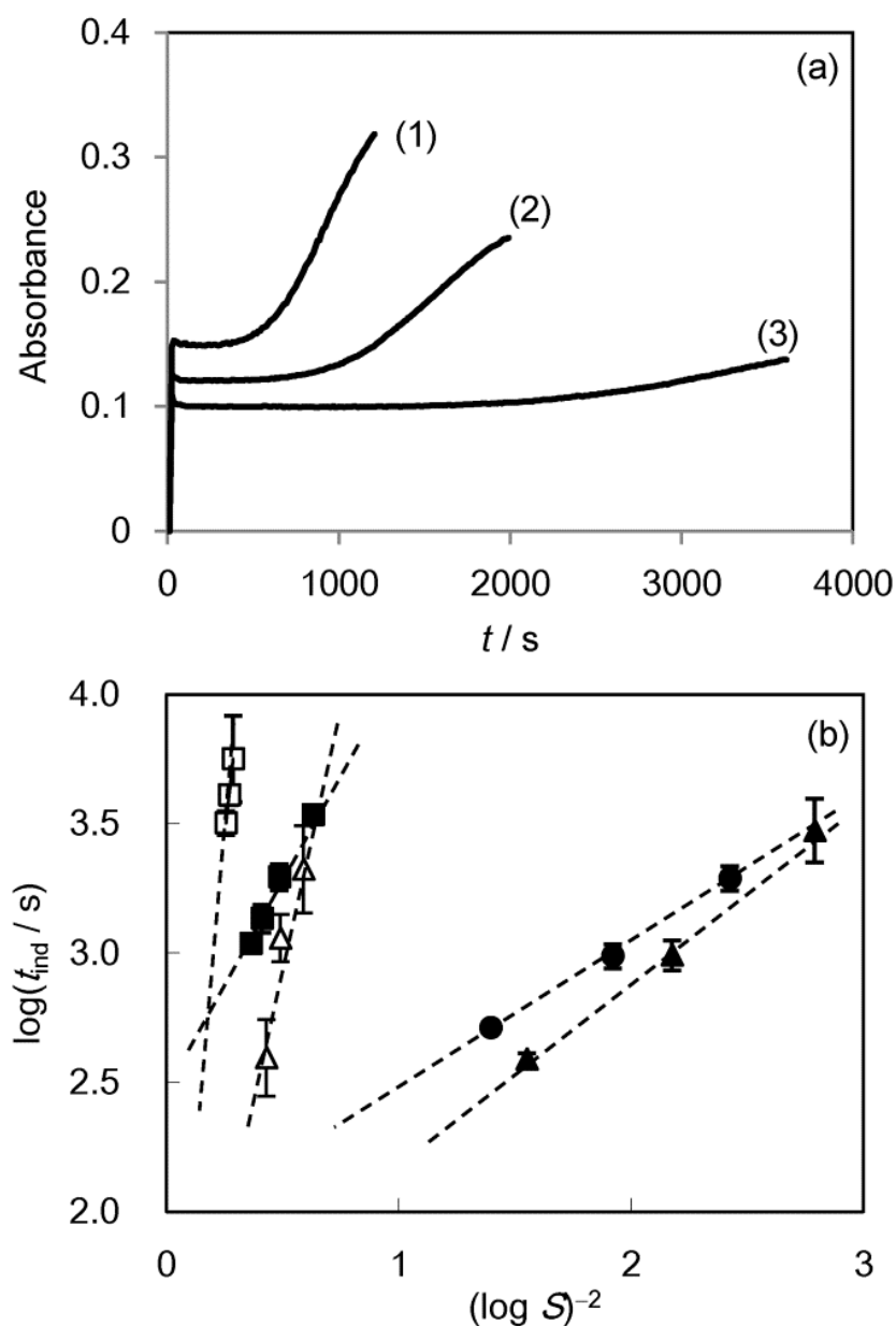
Figure 3.5. (a) Time-absorbance curves of supersaturated solution in the presence of (1) 40, (2) 30, and (3) 25 \mu\text{g mL}^{-1} of danazol and (b) plots of \log t_{\text{ind}} versus (\log S)^{-2} for danazol (●), griseofulvin (▲), itraconazole (Δ), vemurafenib (■) and ER-34122 (□). Each value represents the mean \pm SD ( n = 3 ). The broken lines are the regression lines.
