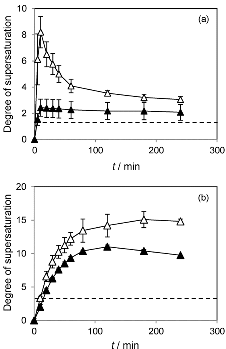
Figure 4.4. The degree of supersaturation versus time profiles of griseofulvin (a) and danazol (b) for pure ( \Delta ) and crystal-contaminated ( \blacktriangle ) amorphous solids in the presence of HPMC. Each value represents the mean \pm SD ( n = 3 ). The broken lines represent the R_s values in the absence of polymers and seed crystals.
