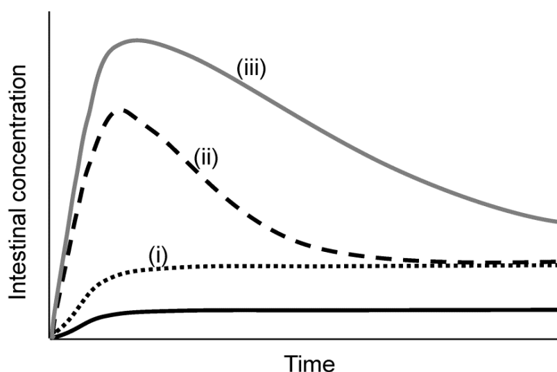
Figure III. Schematic diagrams of time-intestinal drug concentration curves for a poorly soluble drug candidate (black solid curve). (i) Improving thermodynamic solubility by structural modification is the simplest approach to increase average intestinal concentration ( C_{\text{intestine}} ). (ii) Metastable forms such as amorphous forms, salts and cocrystals induce supersaturation and show higher apparent solubility than thermodynamic solubility. (iii) Crystallization inhibitors can further improve supersaturation profiles of the metastable forms.
