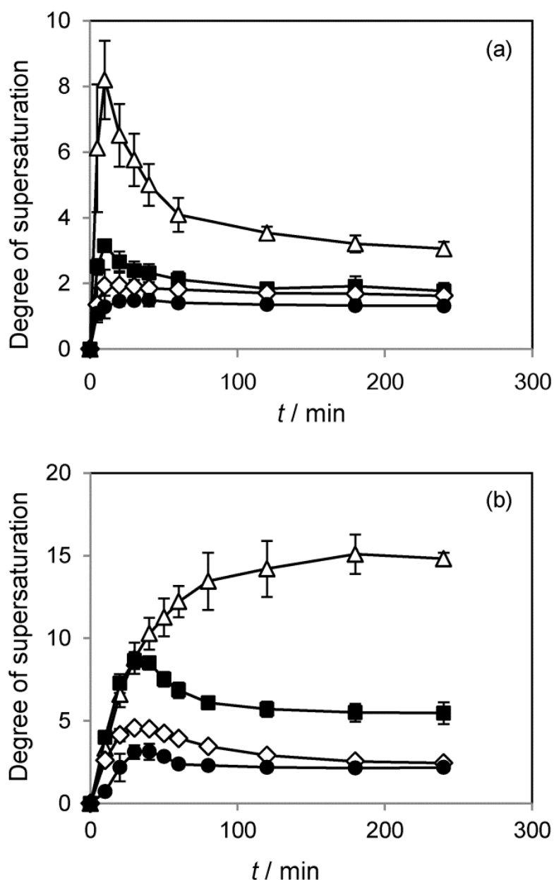
Figure 4.1. The degree of supersaturation versus time profiles of amorphous griseofulvin (a) and danazol (b) in dissolution tests in the absence of polymers (●) and in the presence of HPMC (Δ), PVP (■) and Eudragit (◇). Each value represents the mean \pm SD (n = 3).
