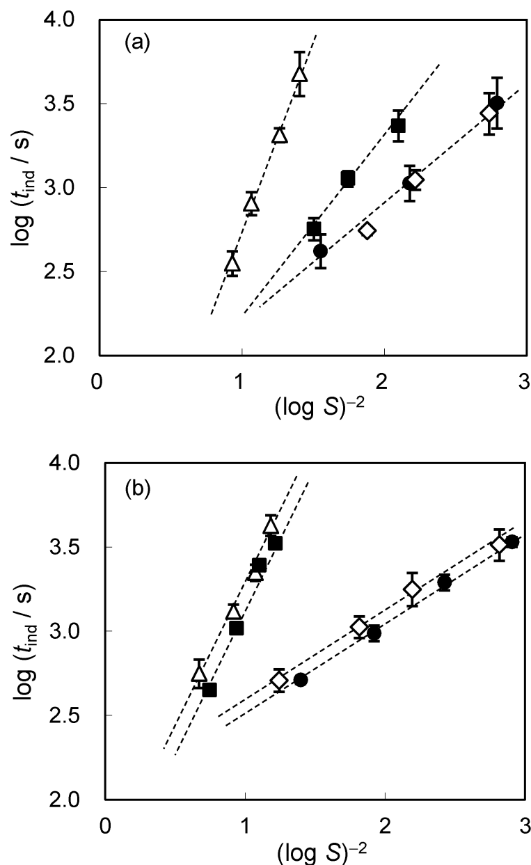
Figure 4.2. Plots of \log t_{\text{ind}} versus (\log S)^{-2} for griseofulvin (a) and danazol (b) in the absence of polymers (●) and in the presence of HPMC (Δ), PVP (■) and Eudragit (◇). Each value represents the mean \pm SD ( n = 3 ).
