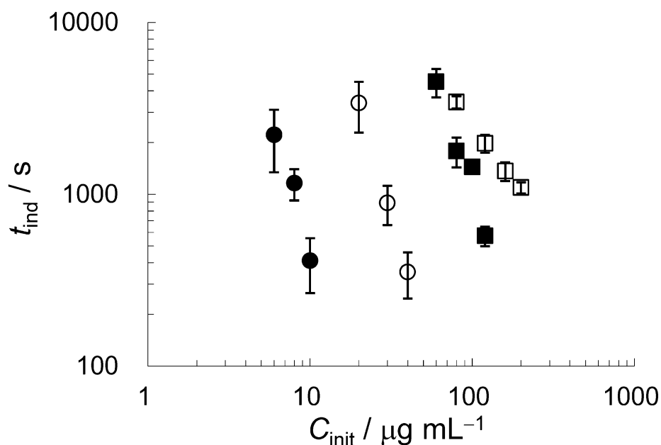
Figure 2.2. Plots of t_{ind} versus C_{init} for itraconazole (●), erlotinib (○), troglitazone (■) and vemurafenib (□). Each value represents the mean \pm SD (n=3).
