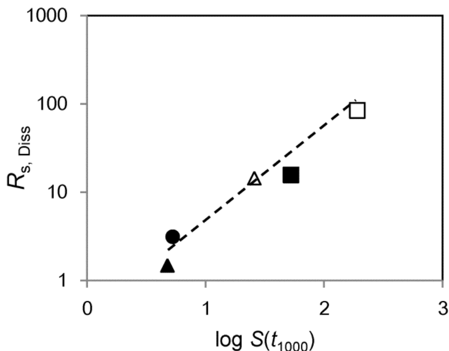
Figure 3.6. Plots of \log R_{s, \text{Diss}} versus \log S(t_{1000}) for danazol (●), griseofulvin (▲), itraconazole (Δ), vemurafenib (■) and ER-34122 (□). The broken line represents the regression line. Vemurafenib is excluded from the regression analysis because its supersaturation is thermodynamically controlled.
