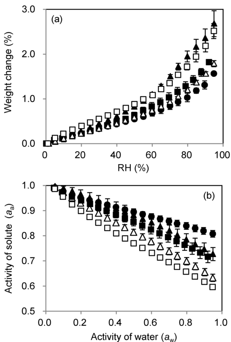
Figure 3.4. (a) Water absorption isotherms and (b) plots of solute activity in amorphous solids for danazol (●), griseofulvin (▲), itraconazole (Δ), vemurafenib (■) and ER-34122 (□).
