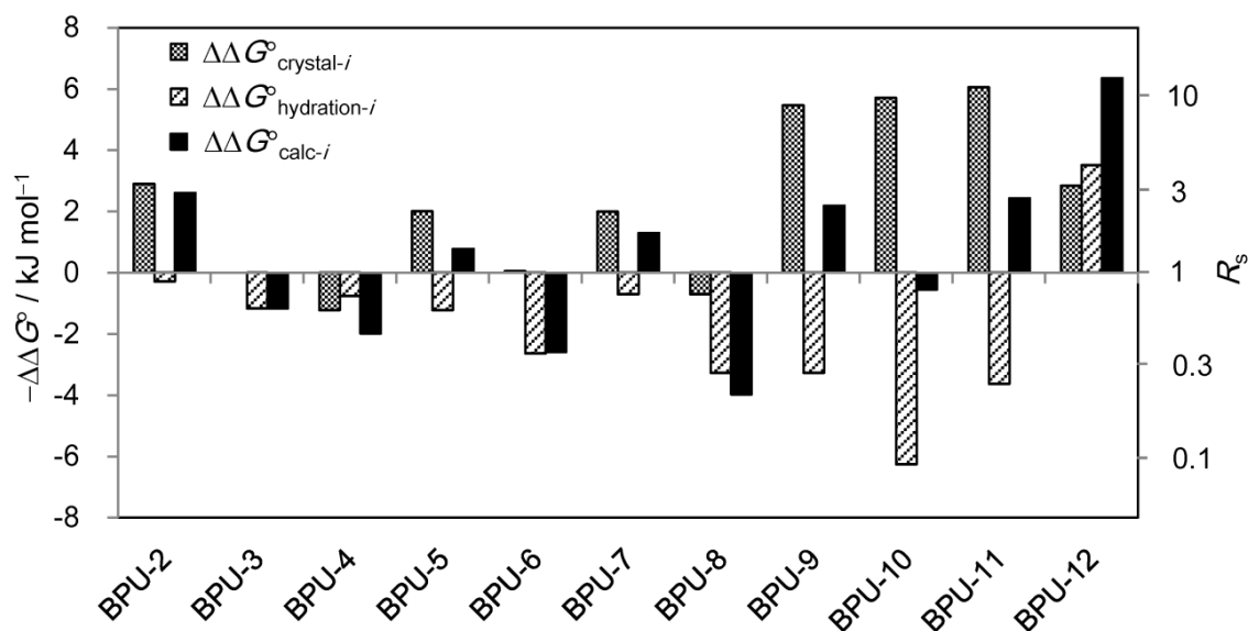
Figure 1.3. The relationships between \Delta\Delta G^\circ_{\text{crystal-}i} , \Delta\Delta G^\circ_{\text{hydration-}i} and \Delta\Delta G^\circ_{\text{calc-}i} for each BPU. The right axis shows the corresponding R_s ( R_{s, \text{crystal-}i} , R_{s, \text{hydration-}i} and R_{s, \text{calc-}i} ) values.
