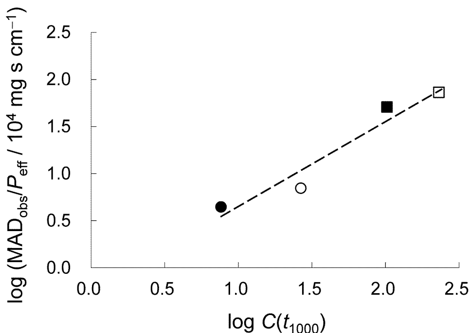
Figure 2.5. Plots of \log (MAD_{obs}/P_{eff}) versus \log C(t_{1000}) for itraconazole (●), erlotinib (○), troglitazone (■), vemurafenib (□). The broken line represents the regression line.
