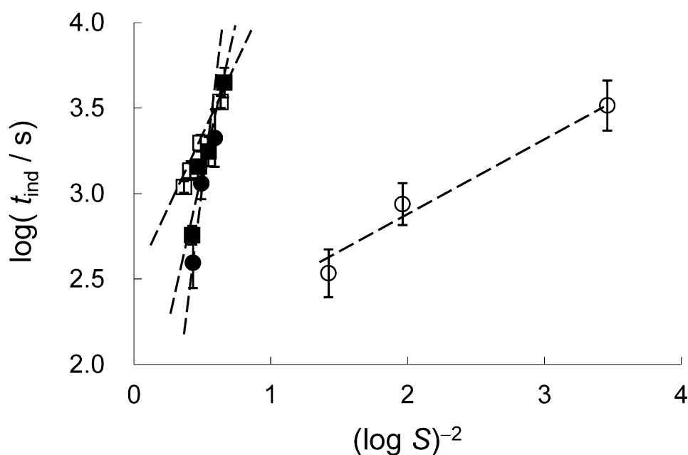
Figure 2.3. Plots of \log t_{\text{ind}} versus (\log S)^{-2} for itraconazole (●), erlotinib (○), troglitazone (■) and vemurafenib (□). Each value represents the mean \pm SD ( n=3 ). The broken lines are the regression lines.
