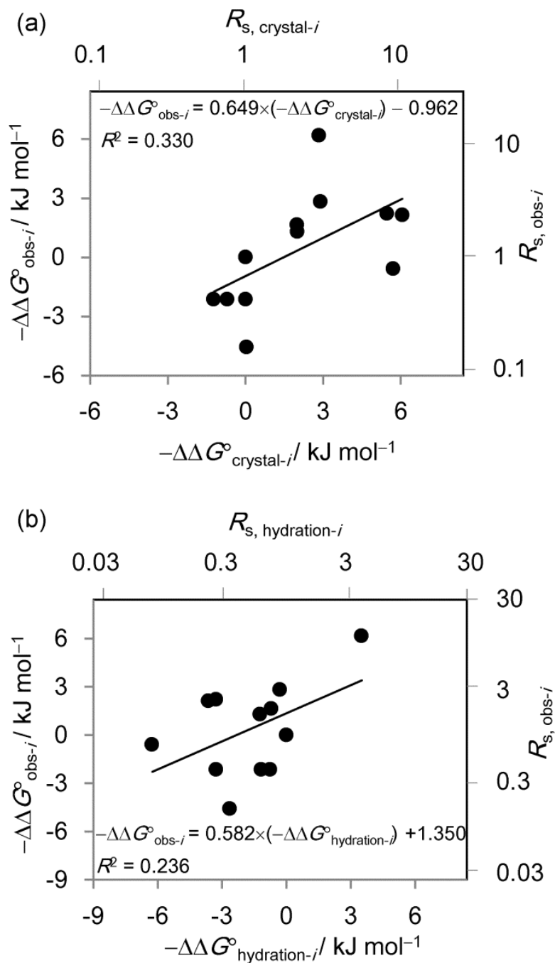
Figure 1.2. (a) Plots of -\Delta\Delta G^\circ_{\text{obs-}i} versus -\Delta\Delta G^\circ_{\text{crystal-}i} for BPUs. The top and right axes show the corresponding R_{s, \text{crystal-}i} and R_{s, \text{obs-}i} values, respectively. (b) Plots of -\Delta\Delta G^\circ_{\text{obs-}i} versus -\Delta\Delta G^\circ_{\text{hydration-}i} for BPUs. The top and right axes show the corresponding R_{s, \text{hydration-}i} and R_{s, \text{obs-}i} values, respectively. The solid lines represent the regression lines.
