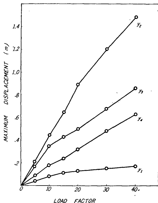
Fig. 11. Maximum Displacements.
