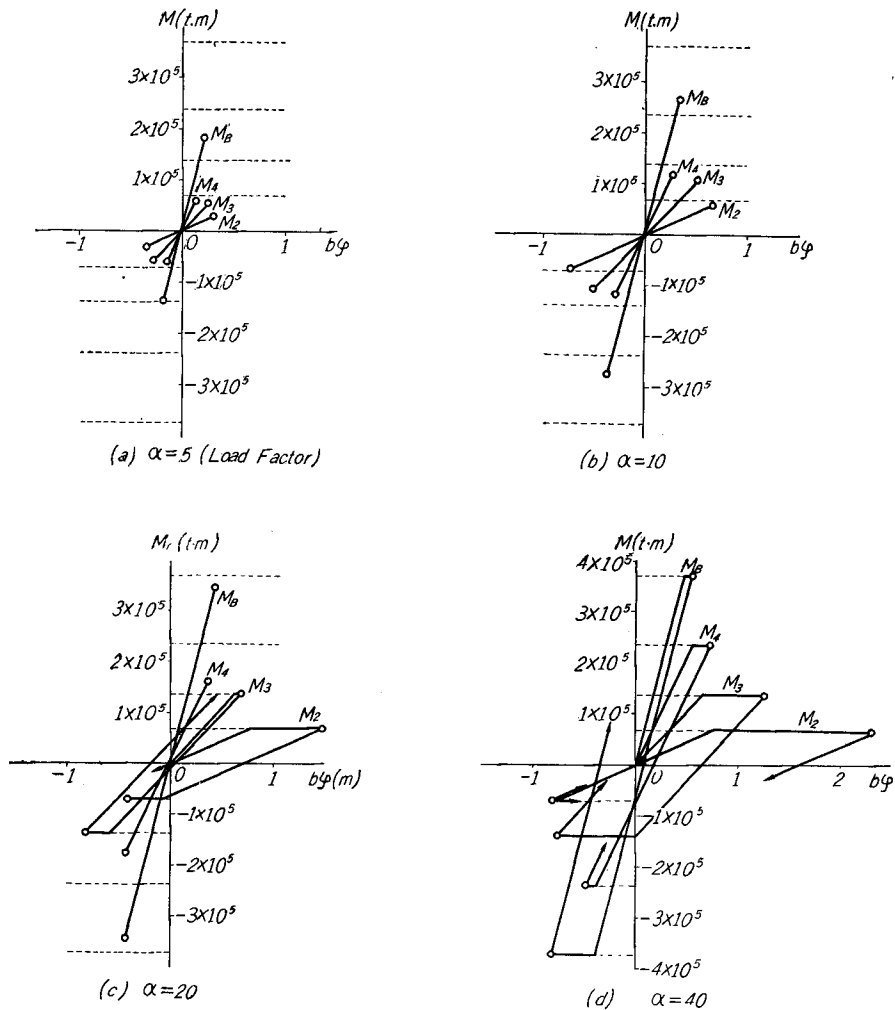
Fig. 13. Hysteresis Curves.
