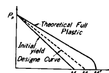
Fig. 2. Interaction Curve for the Tower.
