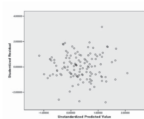
Figure 5. Studentized residuals vs. unstandardized predicted values
