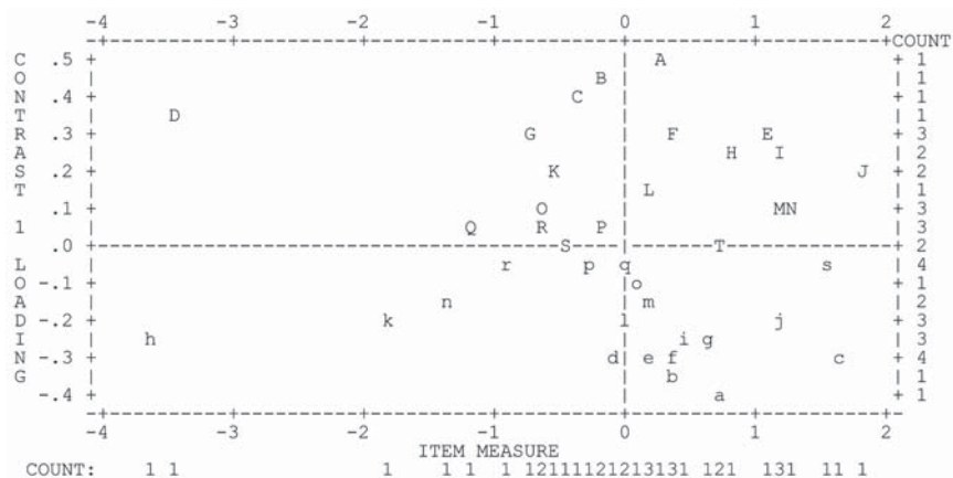
Figure 2. Standardized residual contrast 1 plot
