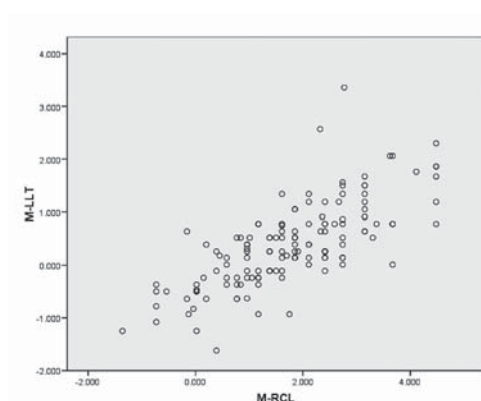
Figure 4. M-LLT vs. M-RCL Plot
