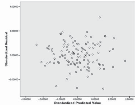
Figure 6. Standardized residuals vs. standardized predicted values
