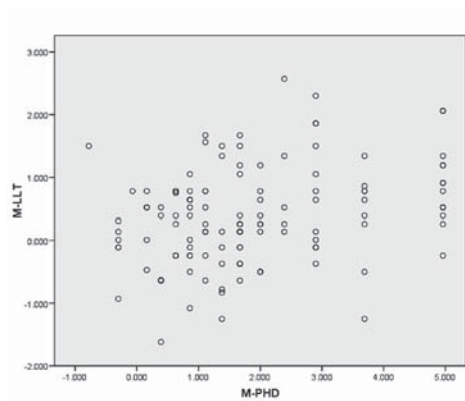
Figure 3. M-LLT vs. M-PHD Plot
