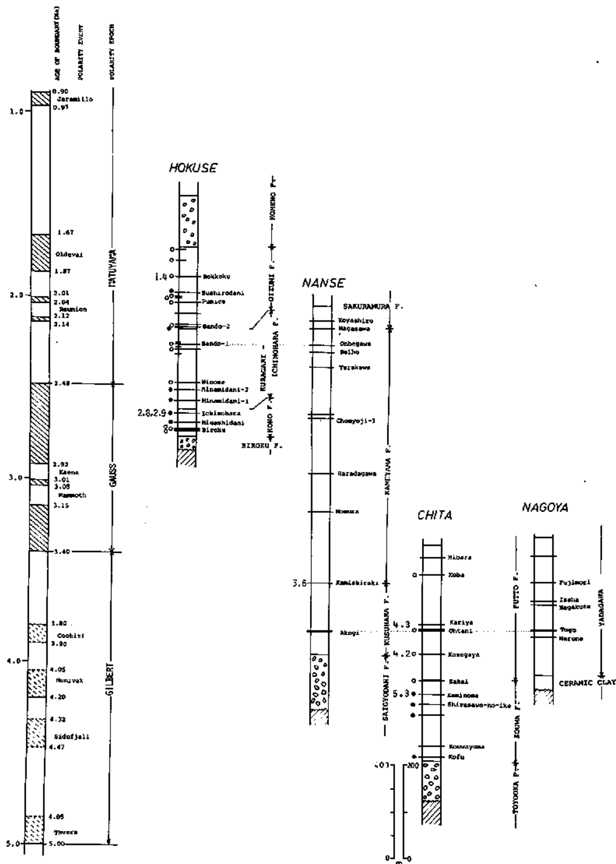
Fig. 33. Correlation chart of the Tokai Group among Hokuse, Nanse, Chita and Nagoya.
