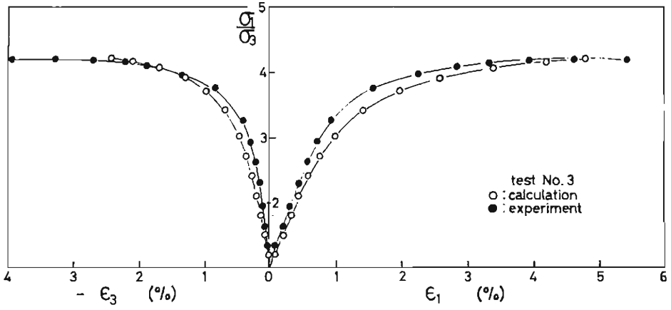
Fig. 8(c) Stress-strain curve obtained from drained triaxial compression test and numerical experiment.
