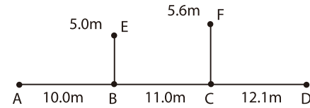
Fig. 1 Transmission line composed of VVF cables.
