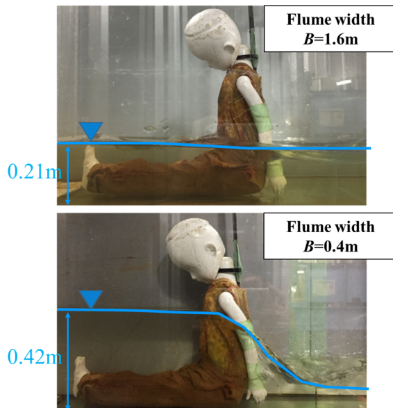
Fig.4 Backwater rise in narrow side ditch
