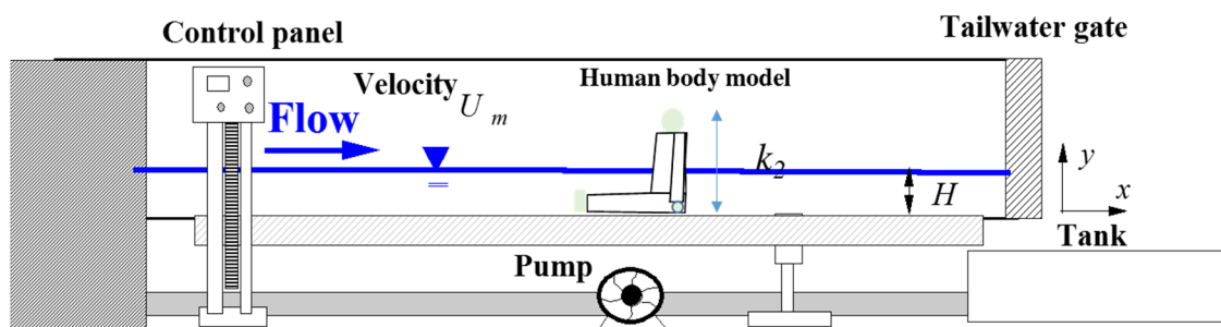
Fig.1 Experimental setup
