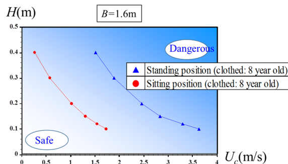
Fig.9 Critical condition for drowning accident (8 year old)
