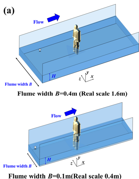
Fig.2(a) Change of flume width
