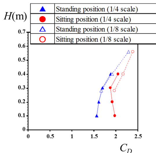
Fig.8 Drag force coefficient of human body in wide open-channel
