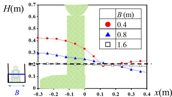
Fig.5 Flow depth change in narrow side ditch
