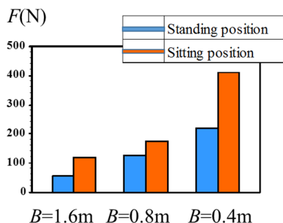
Fig.3 Drag force exerted on human body (effect of flume width)
