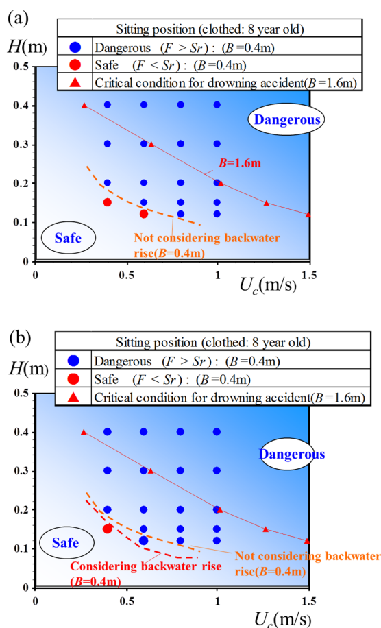
Fig.11 Critical condition for drowning accident in narrow side ditch
