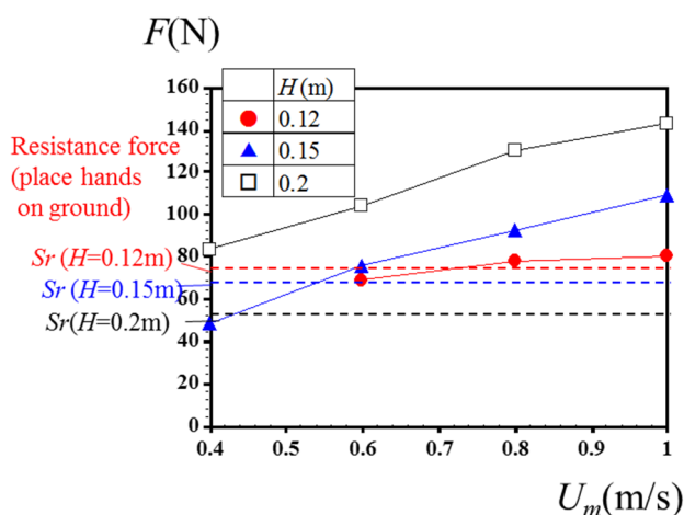
Fig.10 Drag force exerted on human body in narrow side ditch
