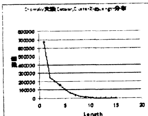
Cluster 2 sentences
