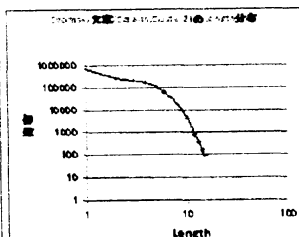
Cluster 2 sentences
