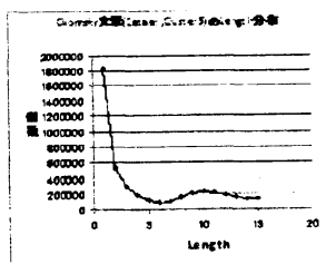
Cluster 5 sentences
