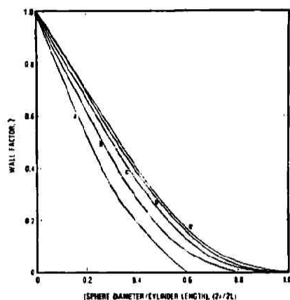
Fig. 13. Dimensionless wall factor \gamma for a right circular cylindrical viscometer of length 2L and radius R in which a sphere of radius a falls along a centrally located diameter. Curve a, R/L=0.6 , curve b, R/L=0.8 , curve c, R/L=1.0 , curve d, R/L=1.2 , curve e, R/L=1.4 .
