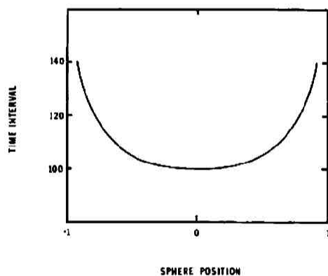
Fig. 14. Idealized graph of the time interval required for a sphere to travel one measuring unit of length at a normalized position in the diamond anvil cell. Arbitrary units are used here.
