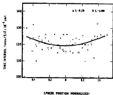
Fig. 15. Central portion of time intervals per measuring unit in (\text{s}/9.47 \times 10^{-1} \text{ cm}) versus normalized sphere position. The center of the cell occurs at position 0 and the boundaries occur at \pm 1 . The solid curve is a least-squares parabola. 2a=0.066 \text{ mm} , 2L=0.169 \text{ mm} , and 2R=0.507 \text{ mm} . Dow-Corning fluid No. 200 is used.
