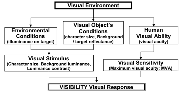
Figure 10: the structure of Visibility Model
