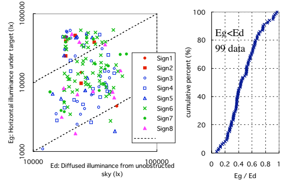
Figure 7-1: E_d and E_g Figure 7-2: E_g/E_d Figure 7: Relationship between Daylight ( E_d ) and Horizontal illuminance under target ( E_g ).
