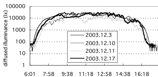
Figure 2: Diffused illuminance from unobstructed sky at latitude 35,02' north and longitude 136,47' east.
