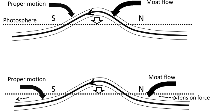
Figure 11. Schematic images of magnetic flux submergence. Top panel illustrates that the moat flows mainly act on the magnetic flux above the solar surface and directly drag the flux downwards. Bottom one shows that the moat flows act on the flux below the surface and enhance the magnetic tension force.
