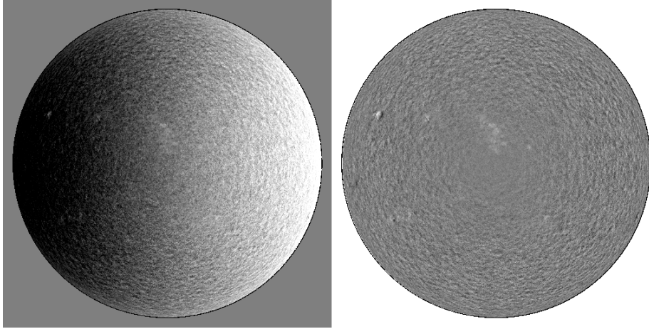
Figure 2. An original MDI Dopplergram (left) and the data after correction for solar rotation and 5 min oscillation (right).
