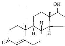
(72)
