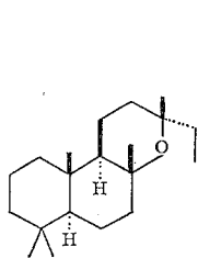
(114)
