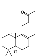
(111)
