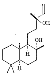
(112)
