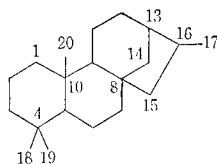
Kaurane
