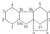
Gibbane
