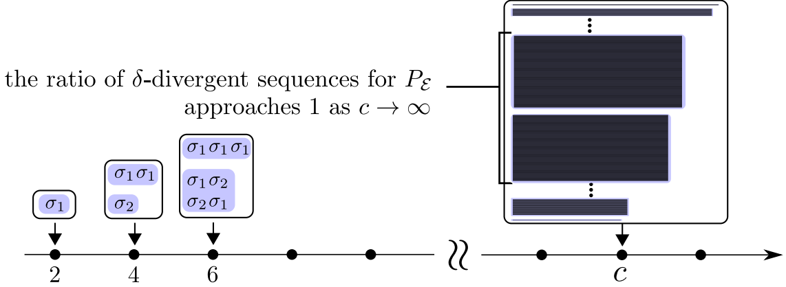
Figure 3.3: Schematic diagram showing that the ratio of \delta -divergent sequences for P_{\mathcal{E}} in W_{\mathcal{E},(c-\Delta c,c]} approaches 1 as c becomes infinite. Here, we consider the symbols \Sigma = \{\sigma_1, \sigma_2\} with energies \mathcal{E}(\sigma_1) = 2 and \mathcal{E}(\sigma_2) = 4 .
