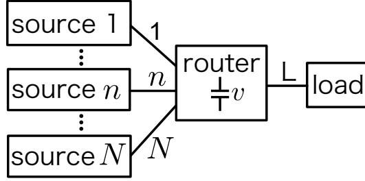
Figure 2.5: Schematic diagram of the system to investigate up-stream dispatching of power at router.
