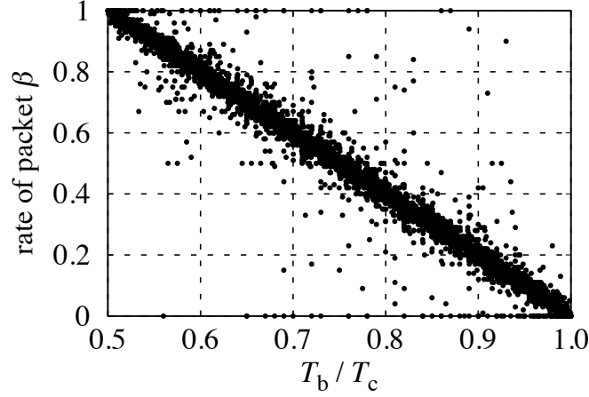
Figure 2.3: Relationship between the ratio T_b/T_c and the rate of packet \beta in 10,000 trials.
