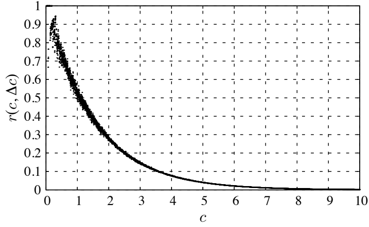
Figure 3.4: r(c, \Delta c) with a change of c .
