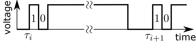
Figure 2.1: Voltage waveform of power packet. Each tag represents “10”, i.e. packet \alpha . The payload is accompanied with the current.
