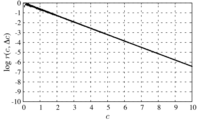
Figure 3.5: \log r(c, \Delta c) with a change of c .
