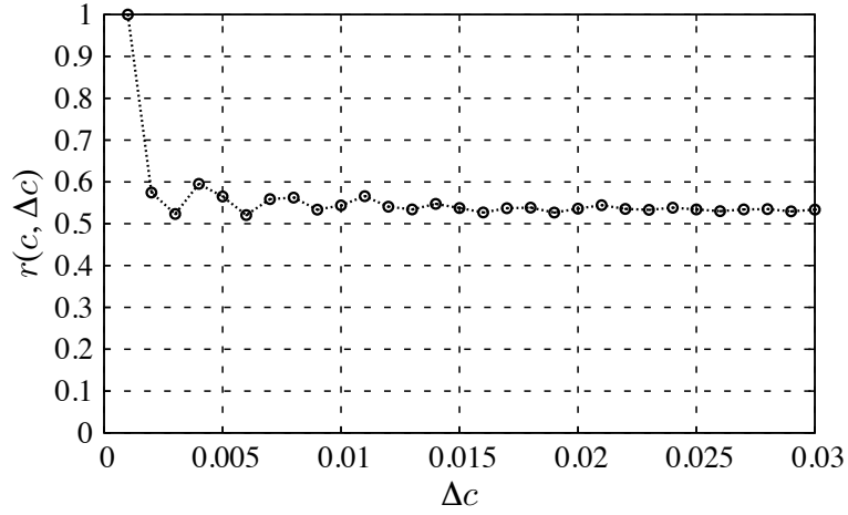
Figure 3.6: r(c, \Delta c) with a change of \Delta c .
