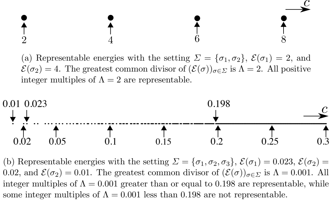
Figure 3.2: Representable energies, i.e. the elements of Eq. (3.3).
