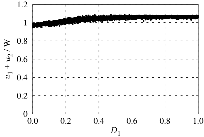
Figure 2.9: Relationship between total amount of transferred power and density of packet 1 in the case of \bar{e}_1^{-1} > \bar{e}_2^{-2} . Only the results which satisfy D_1 + D_2 > 0.3 are plotted to ignore the voltage drop across the capacitor.
