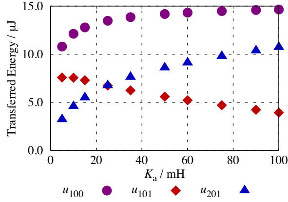
Figure 5.4: The relationship between K_a and energy transferred at the branch point.
