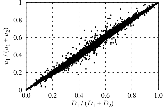
Figure 2.6: Relationship between proportion of transferred power by packet 1 and packet densities in the case of \bar{e}_1^- = \bar{e}_2^- = E_0 .
