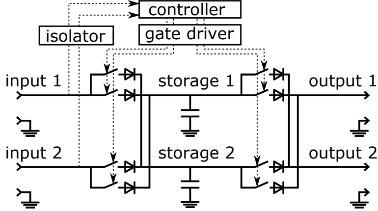
Figure 1.2: Schematic configuration of a router with two inputs, two outputs, and two storage units [42].
