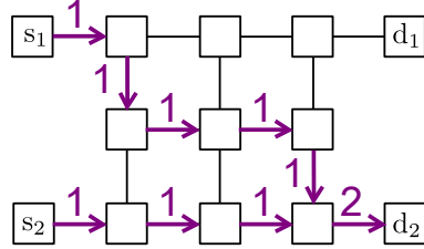
Figure 4.6: An optimal flow in the setting (i) with N = 1 , U_1(s_1) = 1 , U_1(s_2) = 1 , U_1(d_1) = 0 , and U_1(d_2) = -2 , called \alpha_3 .
