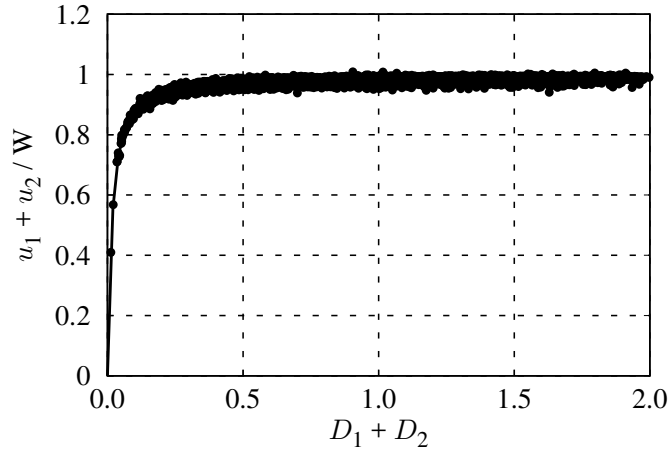
Figure 2.7: Relationship between total amount of transferred power and packet densities in the case of \bar{e}_1^- = \bar{e}_2^- = E_0 . The solid line shows the relationship of Eq. (2.16).
