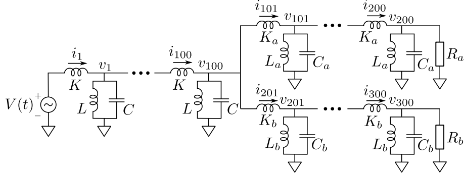
Figure 5.3: A series of inductor-coupled resonator with branch.
