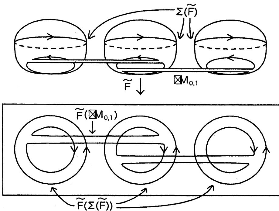
Figure 4: A pseudo-immersion \tilde{F} : M_{0,1} \rightarrow \mathbb{R}^2 .
