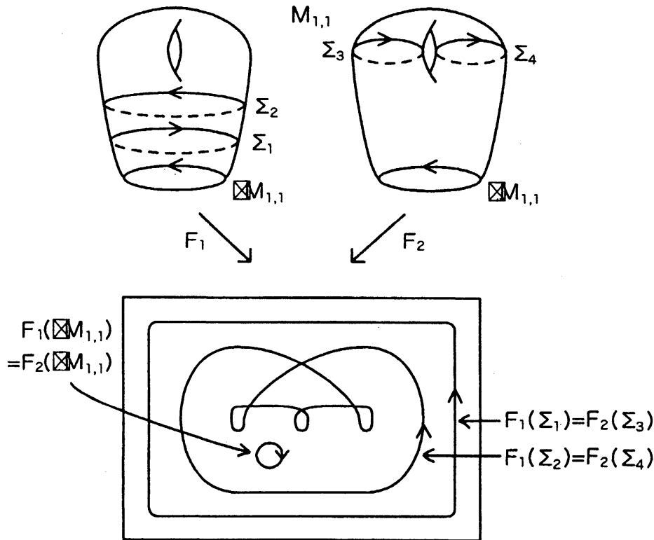
Figure 5: Two pseudo-immersions F_1 and F_2 : M_{1,1} \rightarrow \mathbb{R}^2 such that F_1(\Sigma(F_1)) = F_2(\Sigma(F_2)) .
