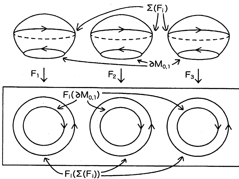
Figure 3: Pseudo-immersions F_i : M_{0,1} \rightarrow \mathbb{R}^2 ( i = 1, 2, 3 ).
