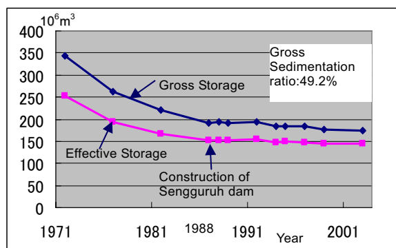
Fig. 2(b) Reservoir sedimentation of Sutami dam
