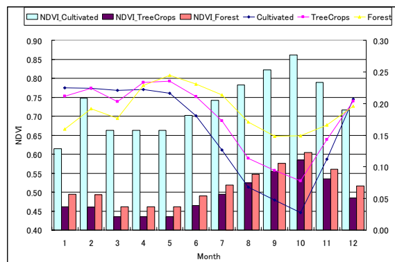
Fig. 15 Seasonal change of the erodibility of the top soil (right) and NDVI (left)
