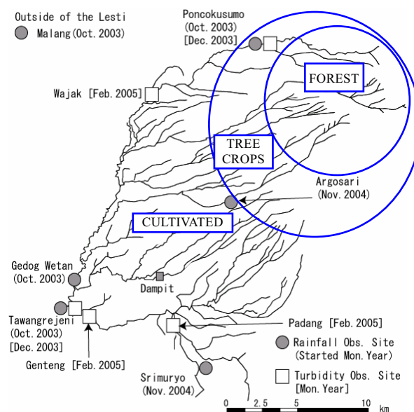
Fig. 3 Observation sites in the Lesti River basin
