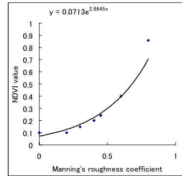
Fig. 18 Relationship between Manning's roughness coefficient and NDVI (NDVI value is obtained from the satellite data taken in December 2002).
