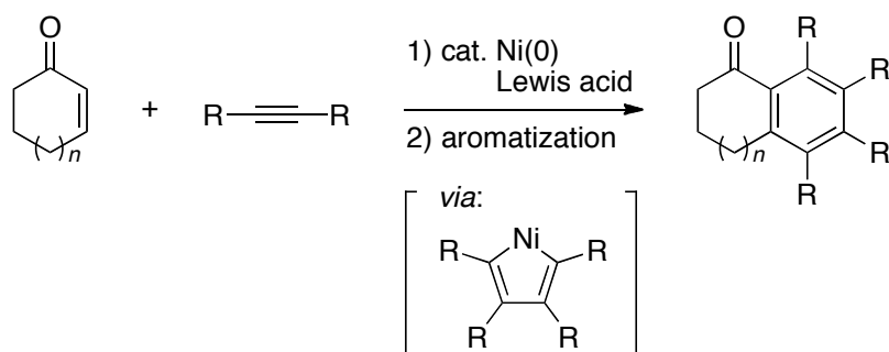
Scheme 8. Nickel-catalyzed [2+2+2] cycloaddition of a cyclic enone with two alkynes.
