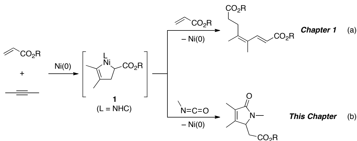
Scheme 1. Formation of nickelacycle 1 and reaction with acrylate or isocyanate.
