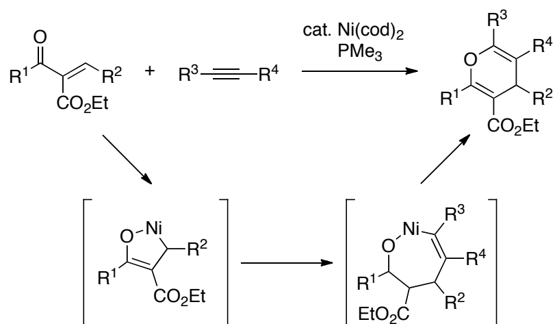
Scheme 10. Nickel-catalyzed [4+2] cycloaddition of enones with alkynes.
