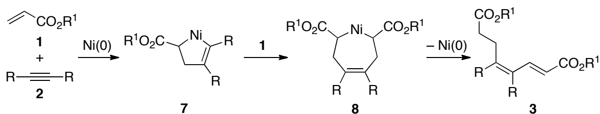
Scheme 2. Plausible reaction mechanism to construct 1,3-diene 3 .
