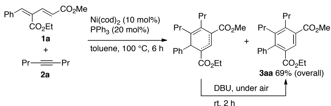
Scheme 2. Nickel-catalyzed [4+2] cycloaddition of diene 1a with alkyne 2a and sequential aromatization.
