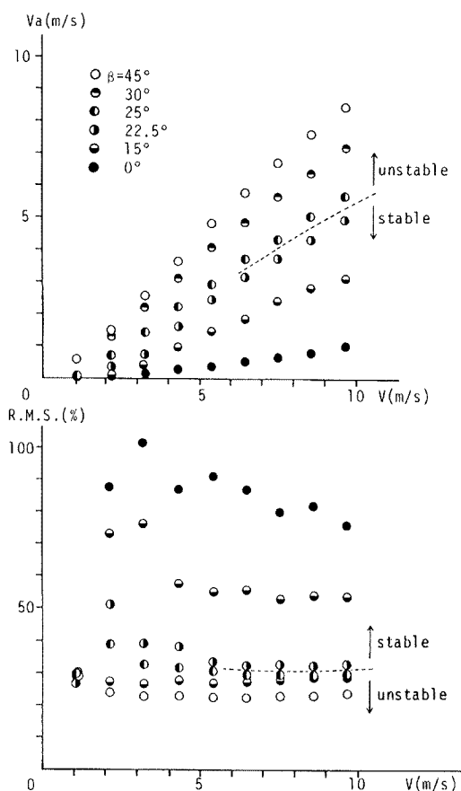
Fig. 12. Velocity characteristics of axial flow ( \alpha=0^\circ , \beta=0^\circ\sim45^\circ ).
