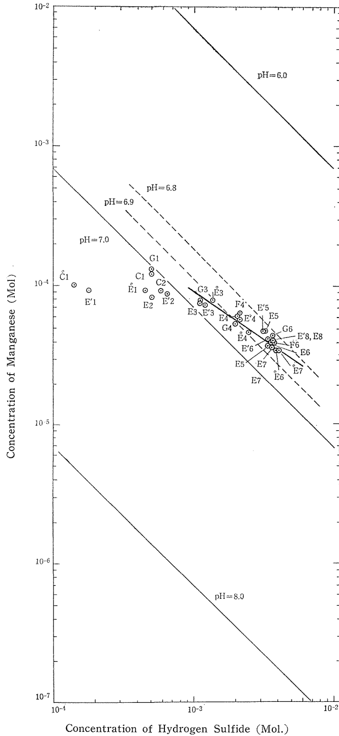
Fig. 10. H_2S-Mn^{++}-pH relation.
