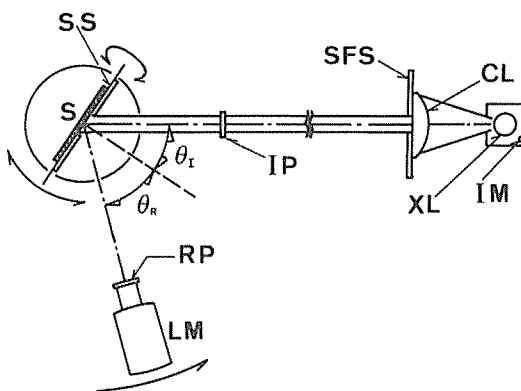
Fig. 3 Optical diagram of goniometric gloss-meter with polarizers. CL: convex lens, IM: illumination photometer, IP: incident polarizer, LM: luminance meter, RP: receptor polarizer, S: specimen, SS: specimen stage, SFS: source field stop, \theta_i : incident angle, \theta_r : receiving angle.
