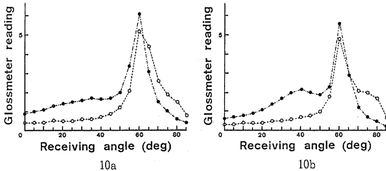
Fig. 10 Goniometric reflection curves — bintangor, microtomed surface, incident angle: 60^\circ . a: LR10°, b: LT10°
