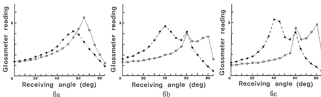
Fig. 6 Goniometric reflection curves — hinoki, incident angle: 60^\circ
