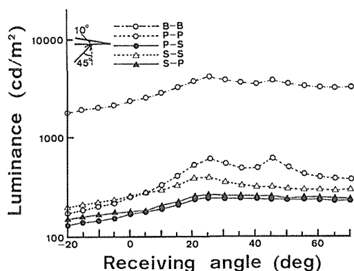
Fig. 8 Goniometric reflection curves measured with polarizers — hinoki: LR10°, microtomed surface.
