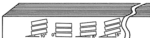
Fig. 1 Diagram for cutting out specimens from lumber.
