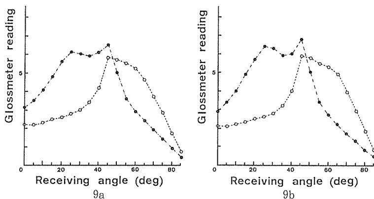
Fig. 9 Goniometric reflection curves — celtis, microtomed surface, incident angle: 45^\circ . a: LR10°, b: LT10°
