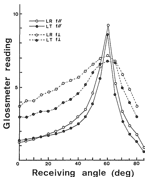
Fig. 4 Anisotropy of reflection - hinoki 0^\circ (LR, LT), incident angle: 60^\circ .: Fiber direction (diving angle) is parallel to the measured surface. LR: LR plane, LT: LT plane, f//: The incident plane is parallel to the grain. f⊥: The incident plane is perpendicular to the grain.
