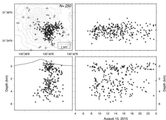
Fig. 8 Spacio-temporal distribution of hypocenters of VT earthquakes of the swarm on August 15, 2015.
