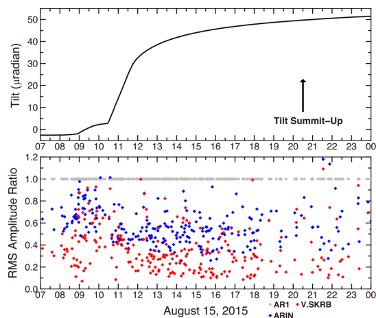
Fig. 9 (top) Record of a water-tube tiltmeter at station AR1. The tiltmeter directs to the crater of Sakurajima. A turning point of the deformation is found at 10:27AM. Stage I is the period before the turning point, while Stage II is the period after the point. (bottom) Relative amplitude ratios of stations ARIN (blue diamond) and V.SKRB (red diamond) with respect to station AR1 (gray diamond).
