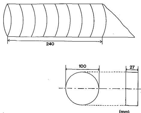
Fig. 3. A typical core sample of rock. Diameter of core samples was 99.3 \pm 0.3 mm and 117.5 \pm 0.4 mm for # 104 to # 133 and for # 154 to # 188, respectively. This is because using two boring cylinders, 100 mm and 120 mm in diameter, were used. Length of core samples was from 200 mm to 450 mm. They were cut into plates about 26.5 \pm 1.5 mm thick except for the surface sections. The cutter produced 0.3 cm-thick cutting losses.
