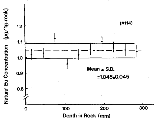
Fig. 4. Stable Eu concentrations at various locations in a core sample (#114). Natural Eu content of the core sample was analyzed by neutron activation methods using the research reactor of Kyoto University (KUR). The mean and standard deviation were 1.045 \pm 0.045 ppm ( \mu\text{g}/\text{lg-rock} ).
