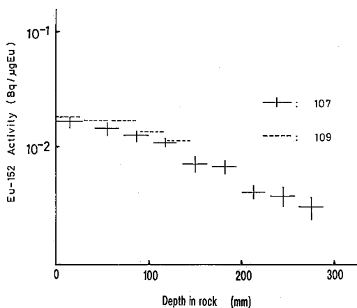
Fig. 10. Figures (A) to (G) show the depth distribution of ^{152}\text{Eu} activities in the rocks. The measured values were normalized per microgram of natural europium and converted to activity at the time of the bombing. Data from samples with their surfaces facing the epicenter taken from the embankment of the Shimono-kawa are plotted in Figures (A) and (B). Data from samples with their surface opposing the epicenter taken from the embankment of the Shimono-kawa are plotted in Figures (C), (D) and (E). Data from samples with their surface facing the epicenter taken from the embankment of the Urakami-gawa are plotted in Figure (F). Data from samples taken from the opposite embankment are plotted in Figure (G).
