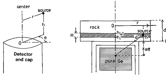
Fig. 9. Parameters for determining of detection efficiency of ^{152}\text{Eu} activity of disk samples.
