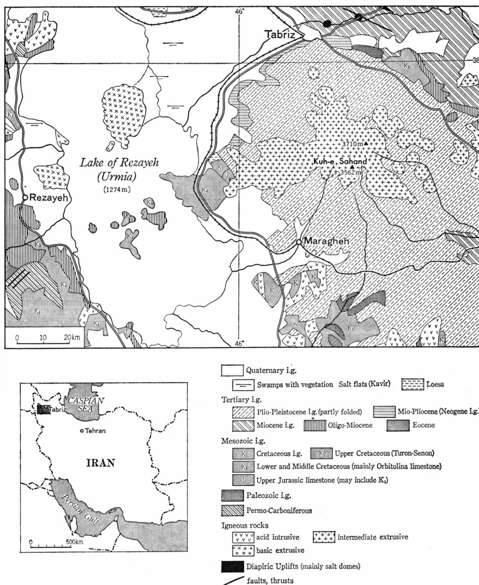
Fig. 1. Index map and Geologic Map of Maragheh Area (from Geological Map of Iran, NIOC 1957)
