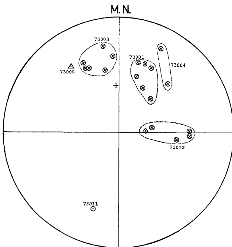
Fig. 15. Directions of NRM's, Schmidt's equal area projection
