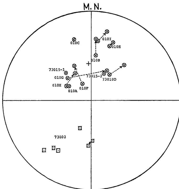
Fig. 16. Directions of NRM
