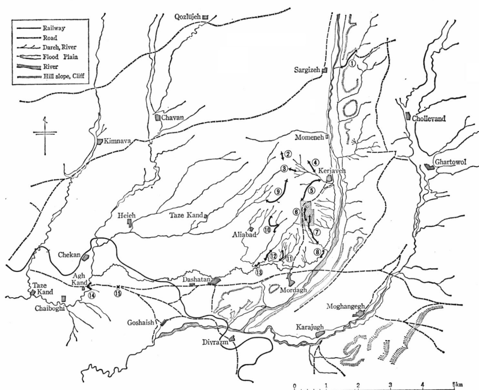
Fig. 3. Map of Surveyed Area and Localities Where Columnar Sections were obtained (1–15 in Fig. 14)
