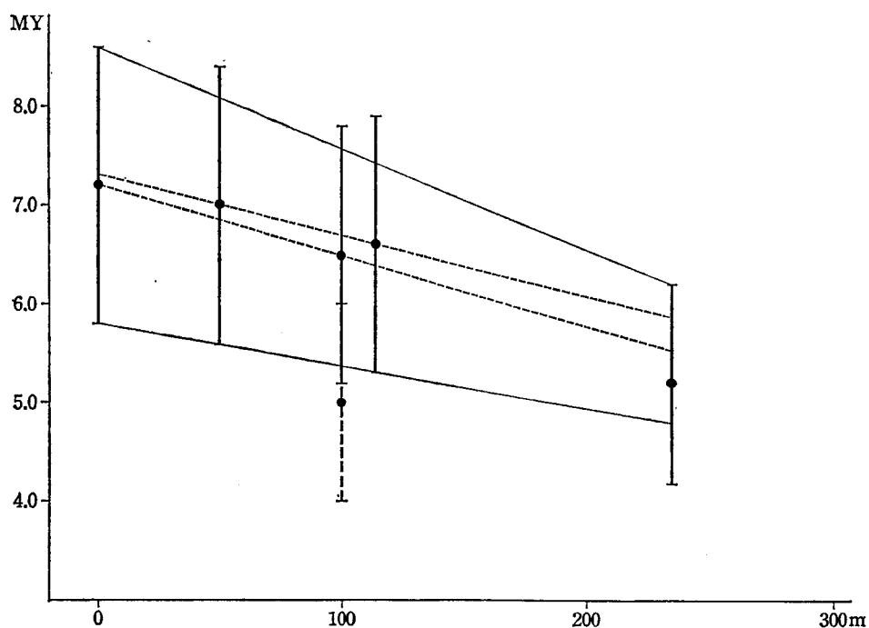
Fig. 17. Fission-track ages and thickness of beds between specimens and base of Maragheh Formation
