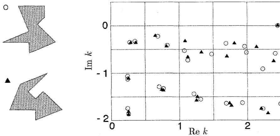
Figure 1. A pair of Isospectral billiards and the distribution of zeros of the Fredholm determinant D(E) on the k(=\sqrt{E}) plane.
