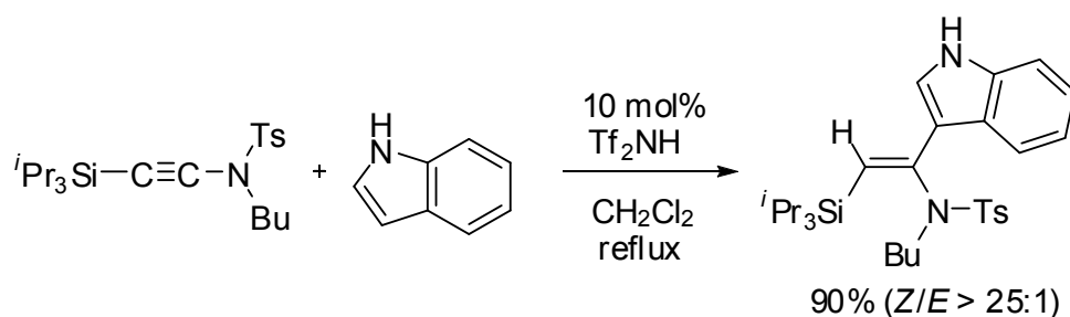
Scheme 33.
