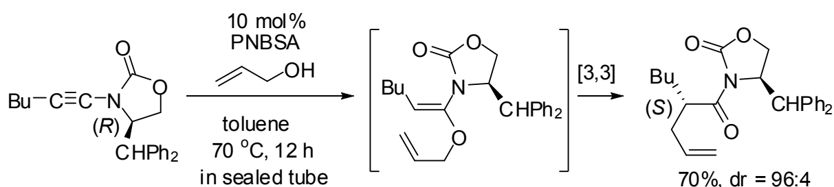
Scheme 32.
