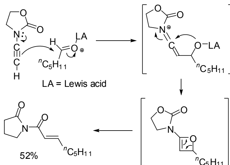
Scheme 34.
