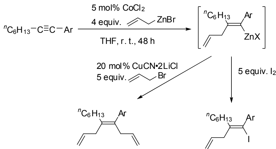
Scheme 37.
