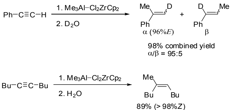
Scheme 5.
