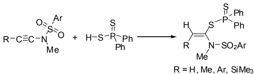
Scheme 44.
