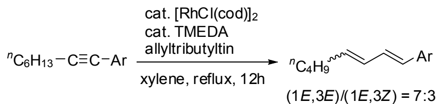
Scheme 38.
