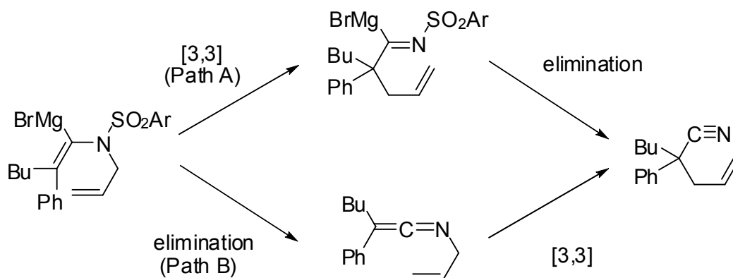
Scheme 43.
